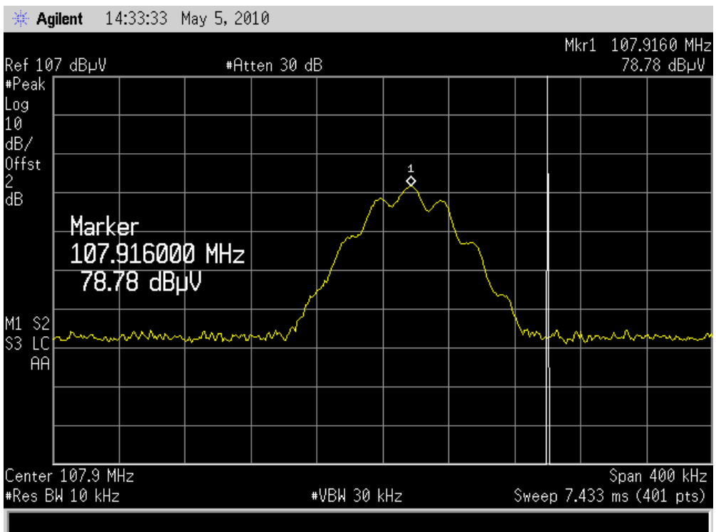
107.9MHZ Test Plot
