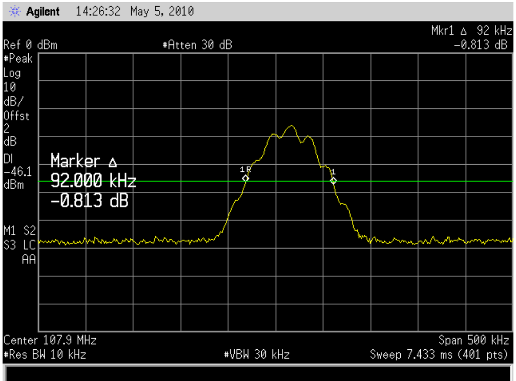
107.9MHZ bandwidth test plot
