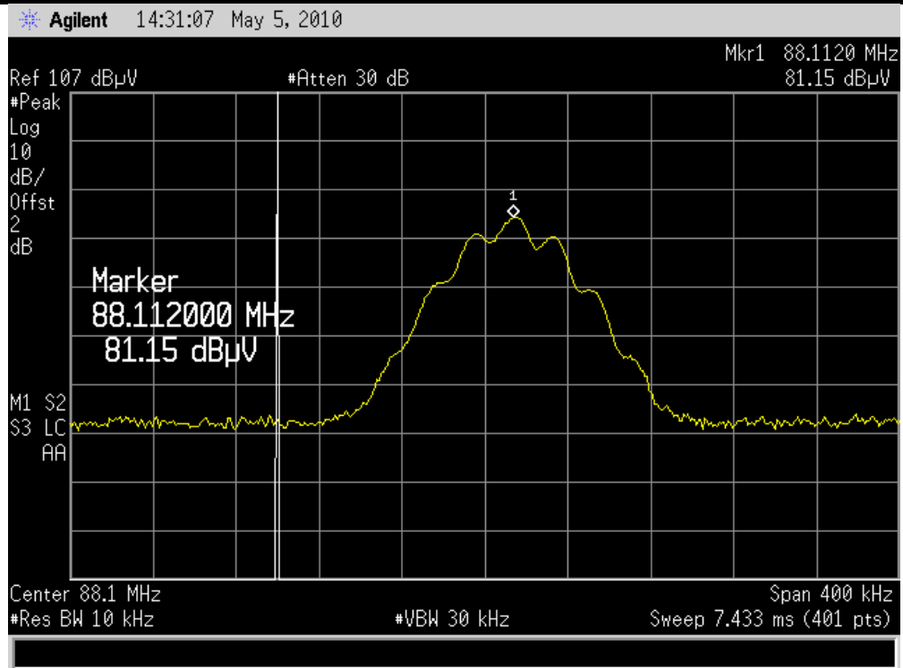
88.1MHZ Test Plot
