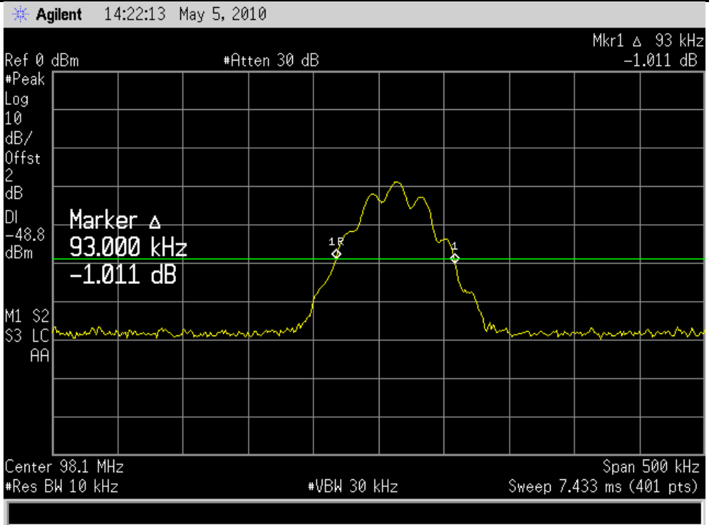
98.1MHZ bandwidth test plot
