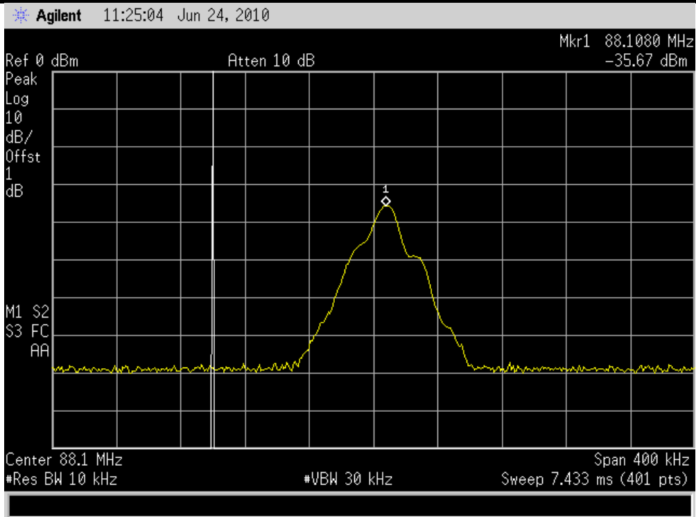
88.1MHz Test Plot
