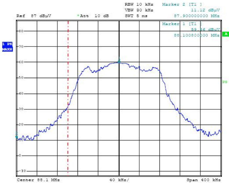
88.1MHz Test Plot
