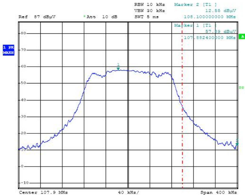
107.9MHz Test Plot
