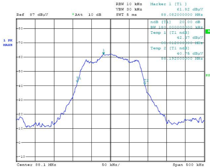
88.1MHZ bandwidth test plot
