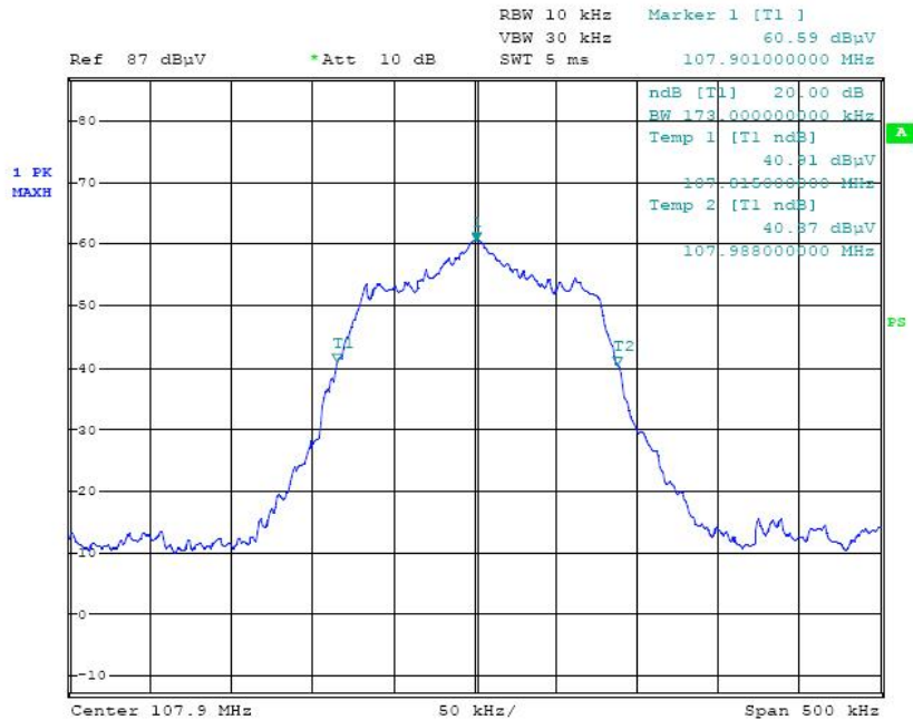
107.9MHZ bandwidth test plot
