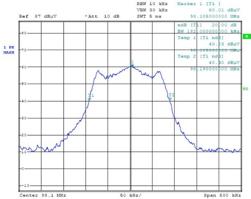
98.1MHZ bandwidth test plot
