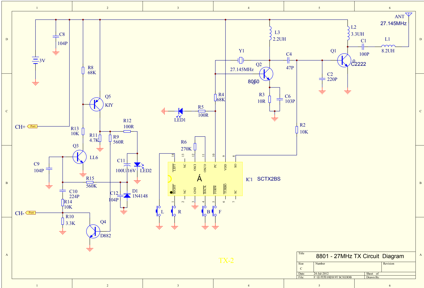
Item No. 8801 - 27MHz Transmitter Circuit Diagram
