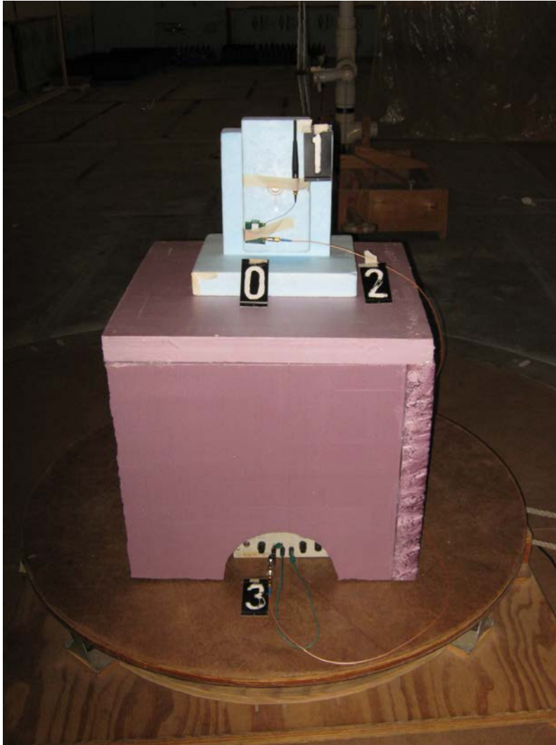
Radiated Emissions below 1 GHz – Position 1
