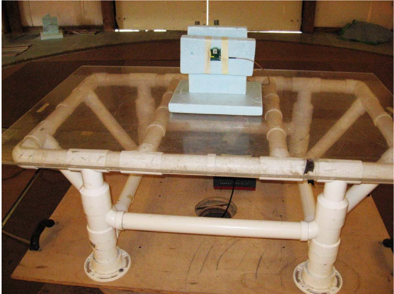
Photo Description: Radiated Emissions Below 1 GHz – X Position
