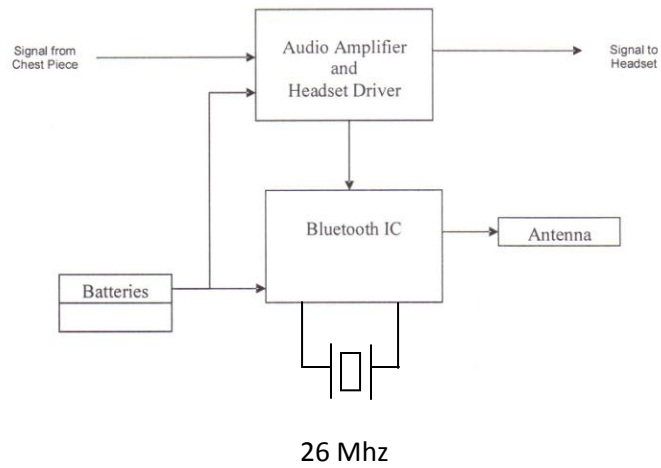
PA/BT Block Diagram March 9, 2009
