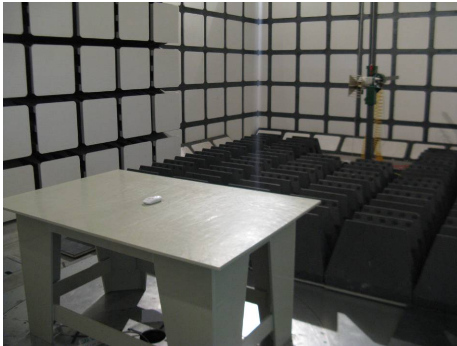
Above 1 GHz: Radiated Emission – Front View (Transmitting mode)
