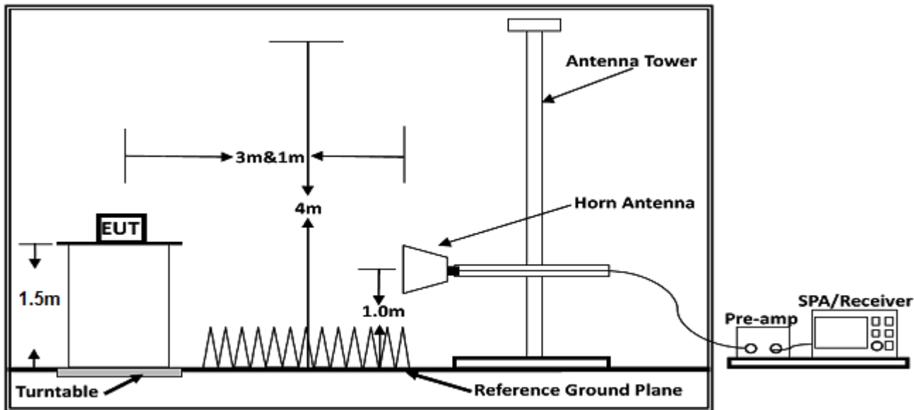
Above 1GHz
