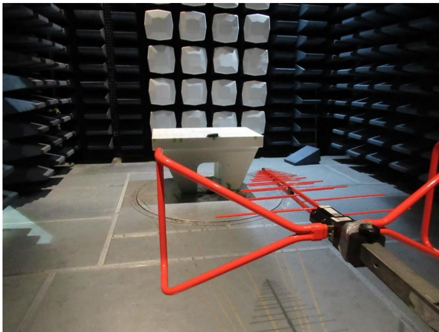
Radiated Emissions performed at the 3m SAC (charging and Battery modes)
