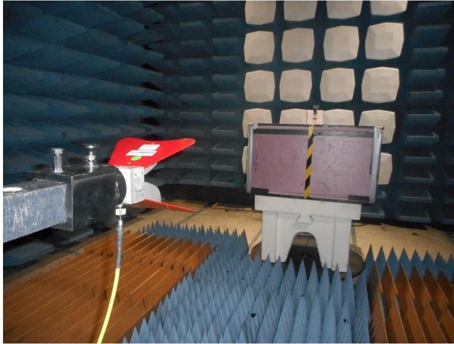
Radiated Emissions performed at the 3m SAC, above 1 GHz
