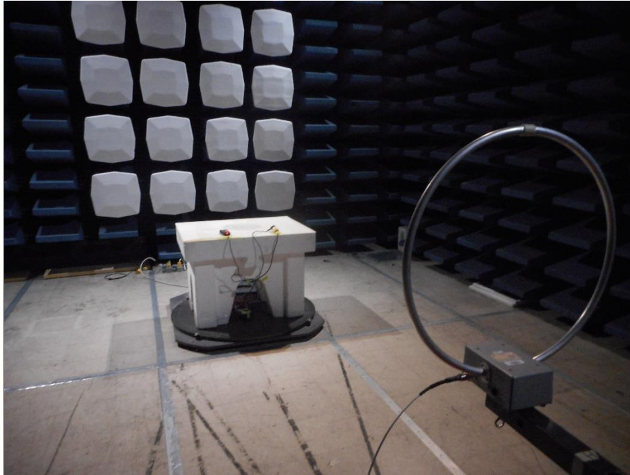
Radiated Emissions performed at the 3m SAC, below 30MHz
