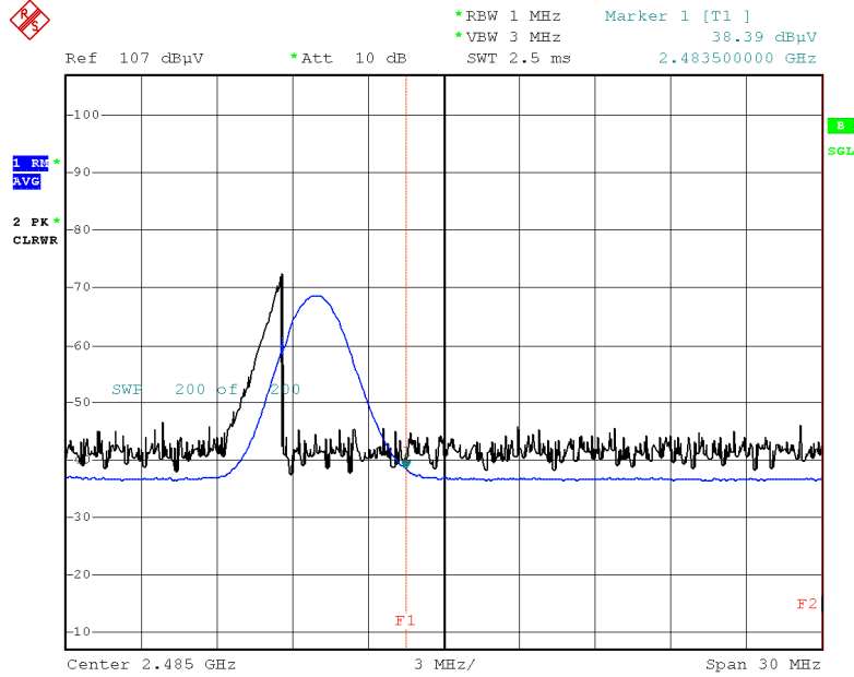
Radiated Restricted Band Edges plot – Average Reading (Ch.39, H)
