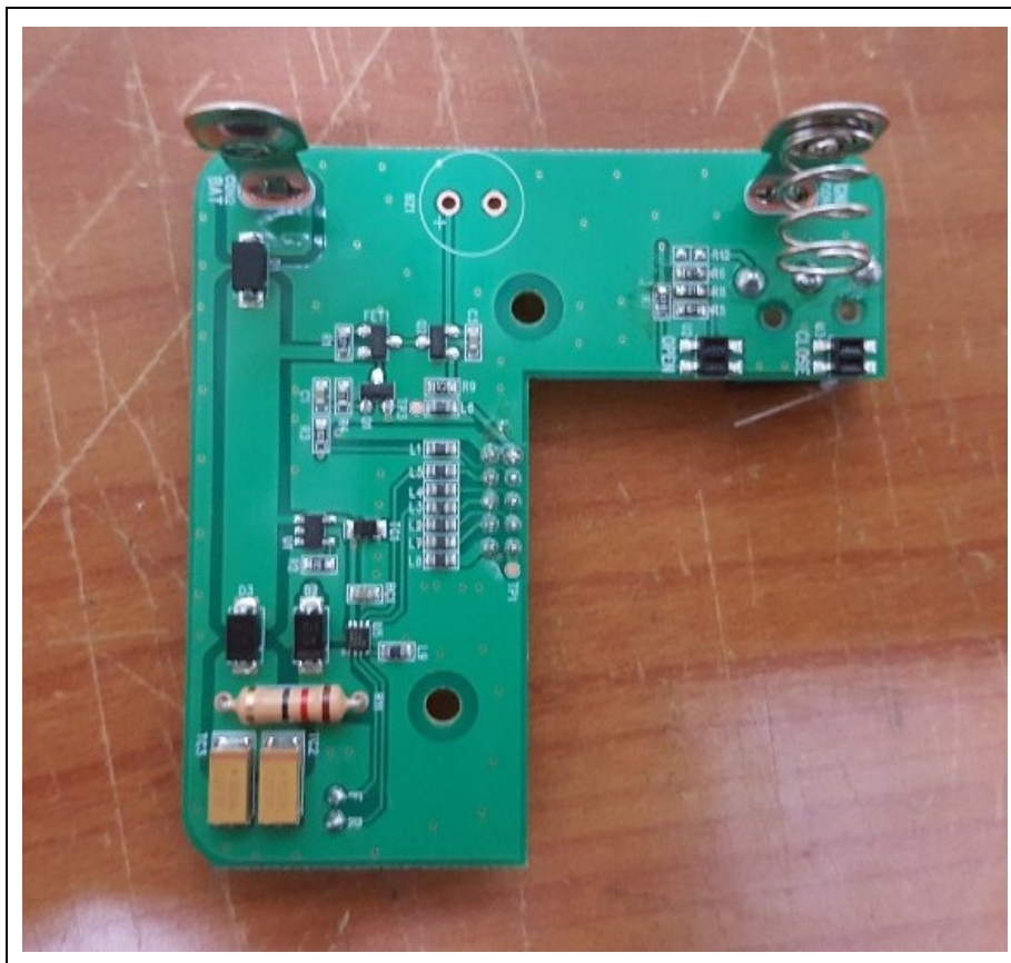
SubBoard-Rear
