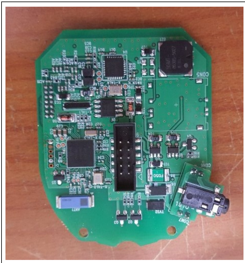
MainBoard-Rear
