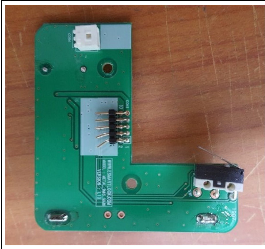
SubBoard-Rear
