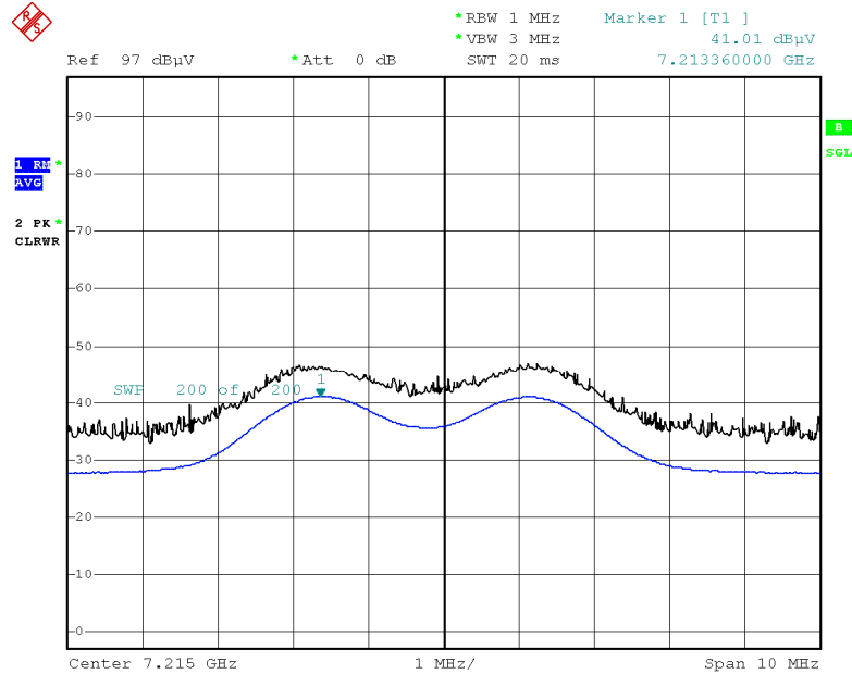
Radiated Spurious Emissions plot – Average Reading (CH.11 3rd Harmonic)
