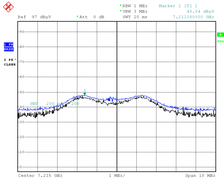
Radiated Spurious Emissions plot – Peak Reading (CH.11 3rd Harmonic)
