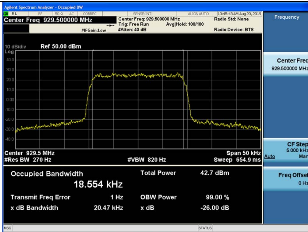
3 dB above the AGC threshold output / 900I_PA(929 ~ 930 MHz) / Downlink
