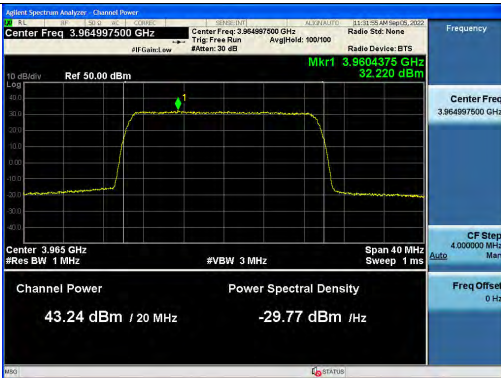
3 dB above the AGC threshold PSD / C-Band(Ant1) / Downlink / 5G NR 20 MHz
