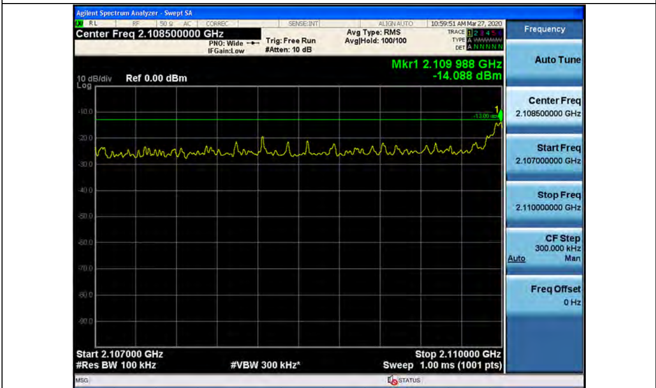
+3 dB above Out-of-band (single test signals) / AWS / Downlink / LTE 10 MHz / Lower
