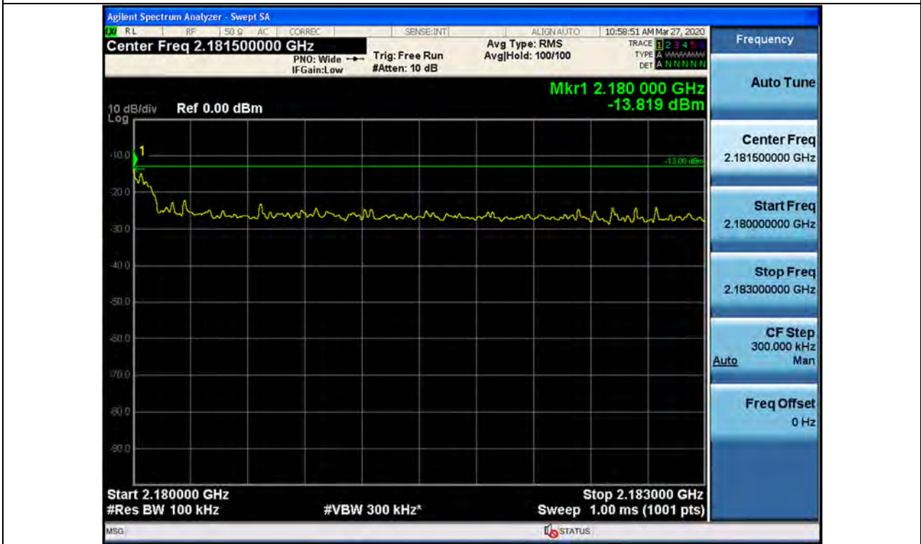
+3 dB above Out-of-band (single test signals) / AWS / Downlink / LTE 10 MHz / Upper
