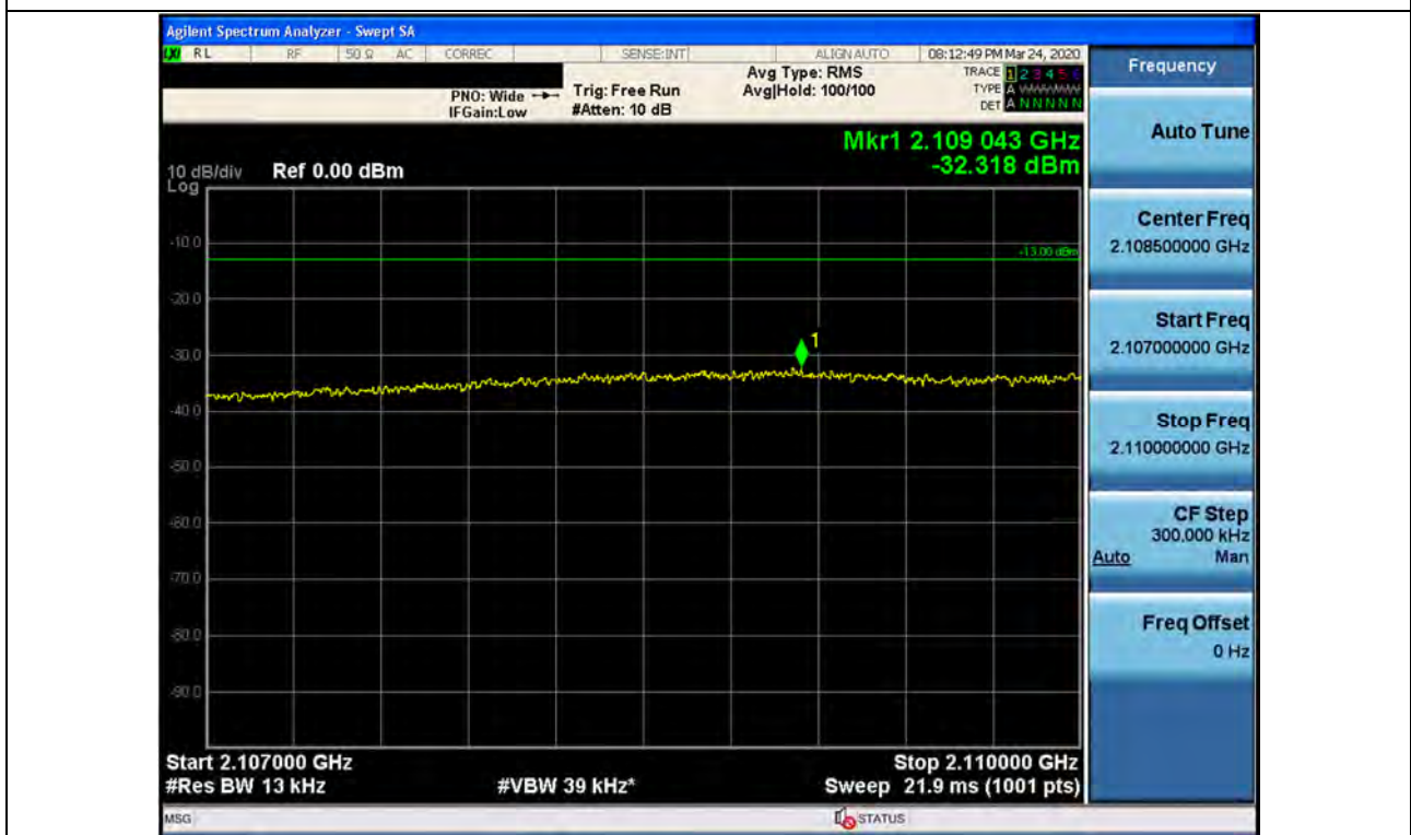
Out-of-band (two adjacent test signals) / AWS / Downlink / CDMA / Lower
