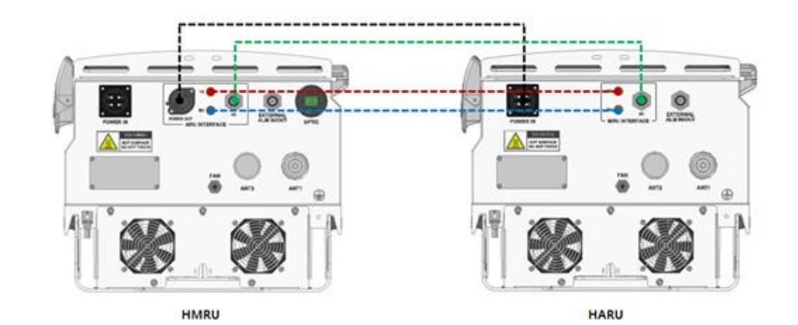
Figure 5.4 – Connecting HMRU with HARU
