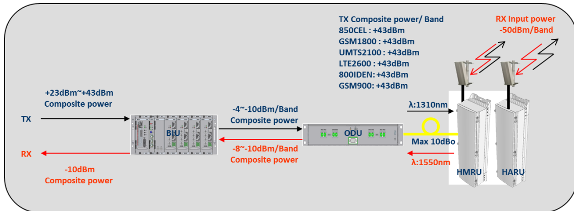
Figure 6.1 – Level Diagram
