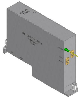
Figure 4.7 – R-Optic Module
