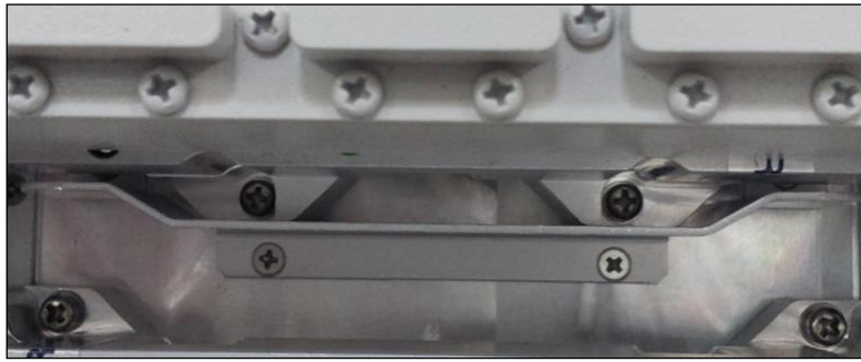
Figure 5.11 – HRDU Installed
