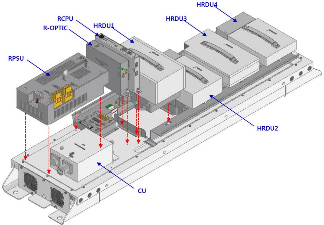
Figure 5.9 – HRDU Configuration
