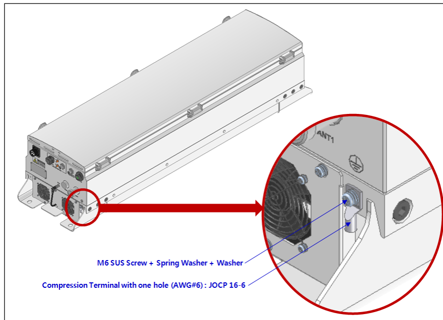
Figure 5.5 – Ground Terminal
