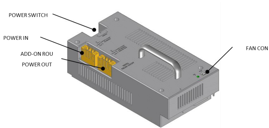
Figure 4.6 – Remote Power Supply Unit
