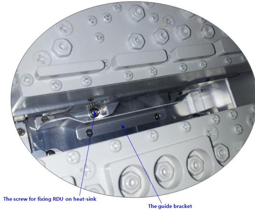
Figure 5.10 – Guide Rail
