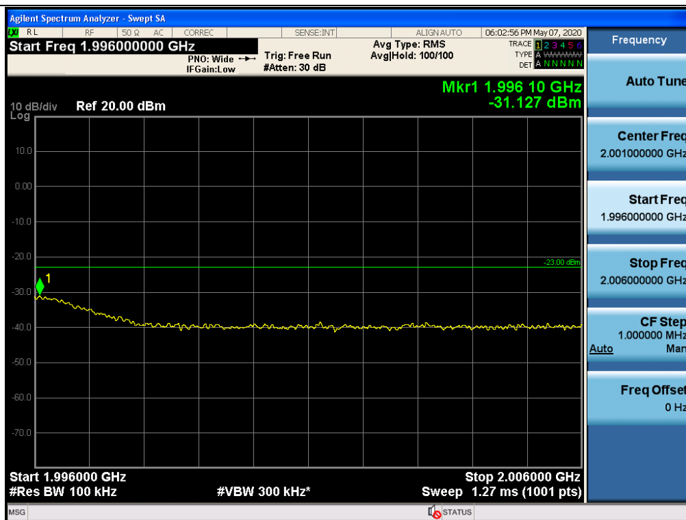
Spurious / PCS / Downlink / GSM / Low / High Edge ~ High Edge+10
