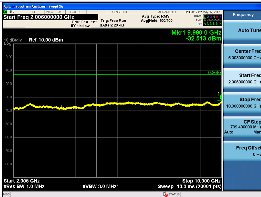
Spurious / PCS / Downlink / GSM / Low / High Edge+10 ~ 10 GHz
