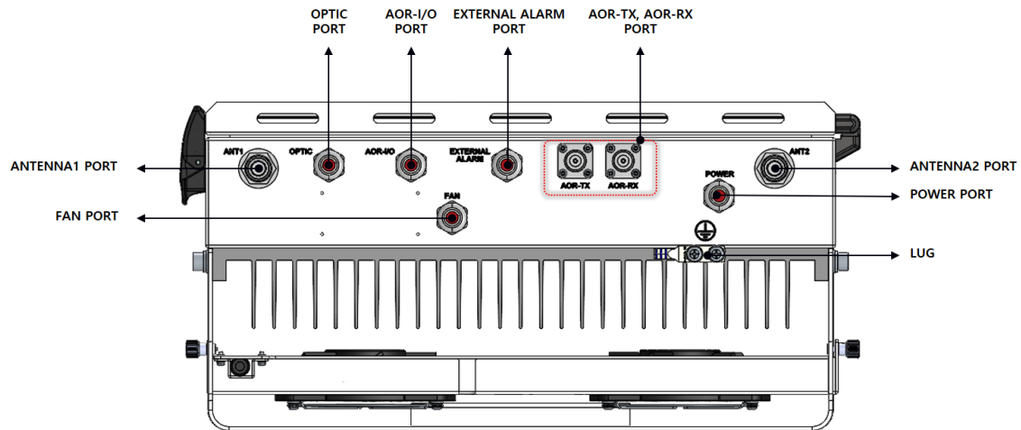
Figure 10. The Bottom Look of HROU_4000
