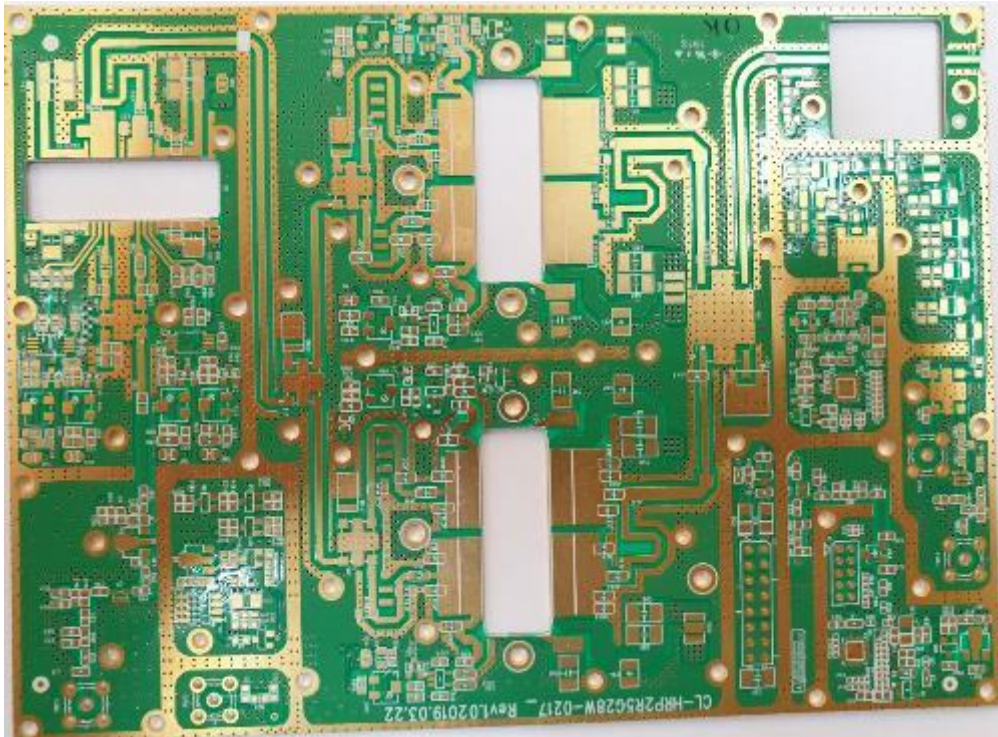
[Main PCB TOP]
