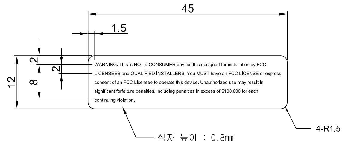
[ Industrial(Part 20) Signal Booster Specifics ]
