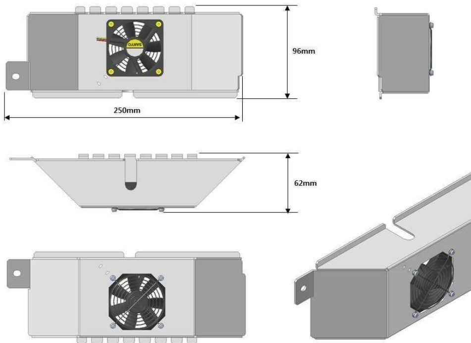
Figure 4.14 – How to mount FAN Unit
