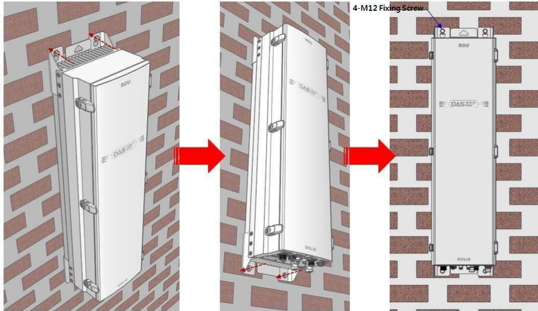
Figure 4.3 – Procedures of installation
