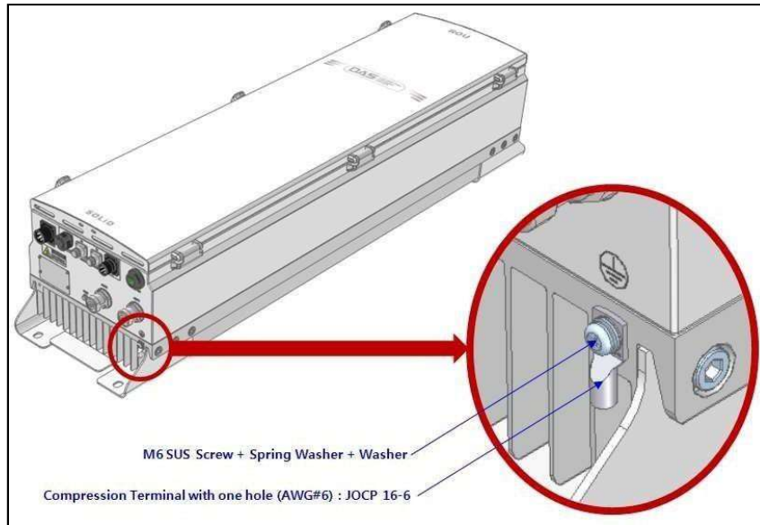
Figure 4.6 – Location of Ground Terminal
