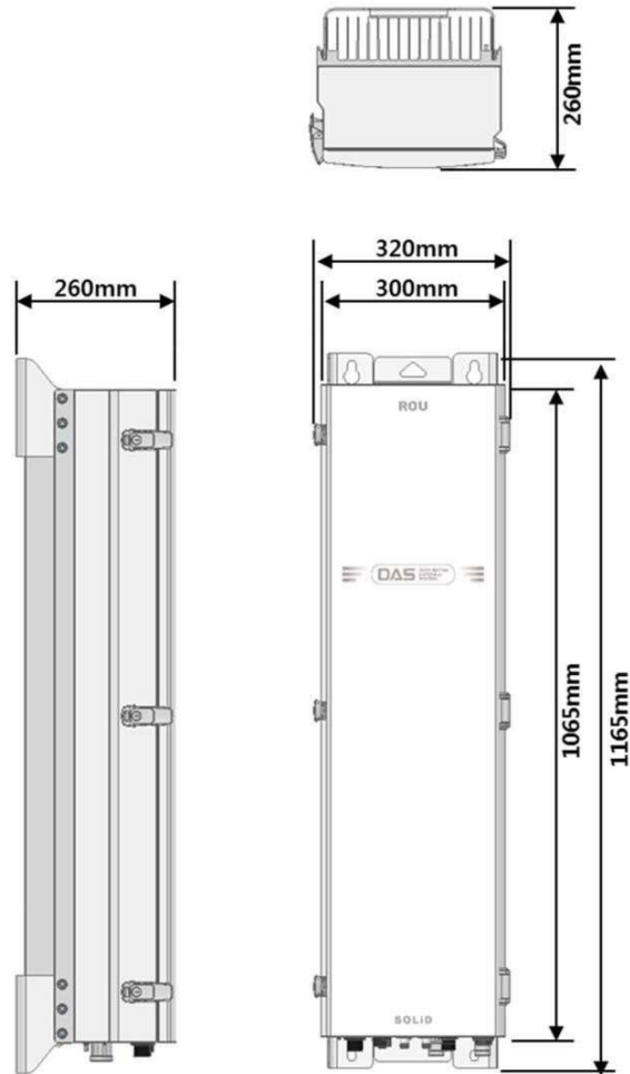
Figure 3.3 – Remote Unit Dimension
