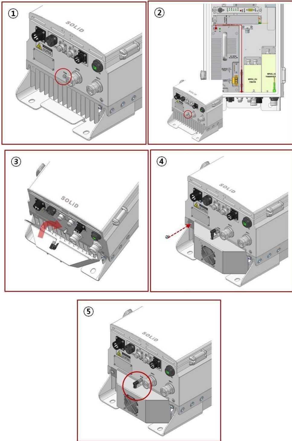
Figure 4.15 – How to mount FAN Unit
