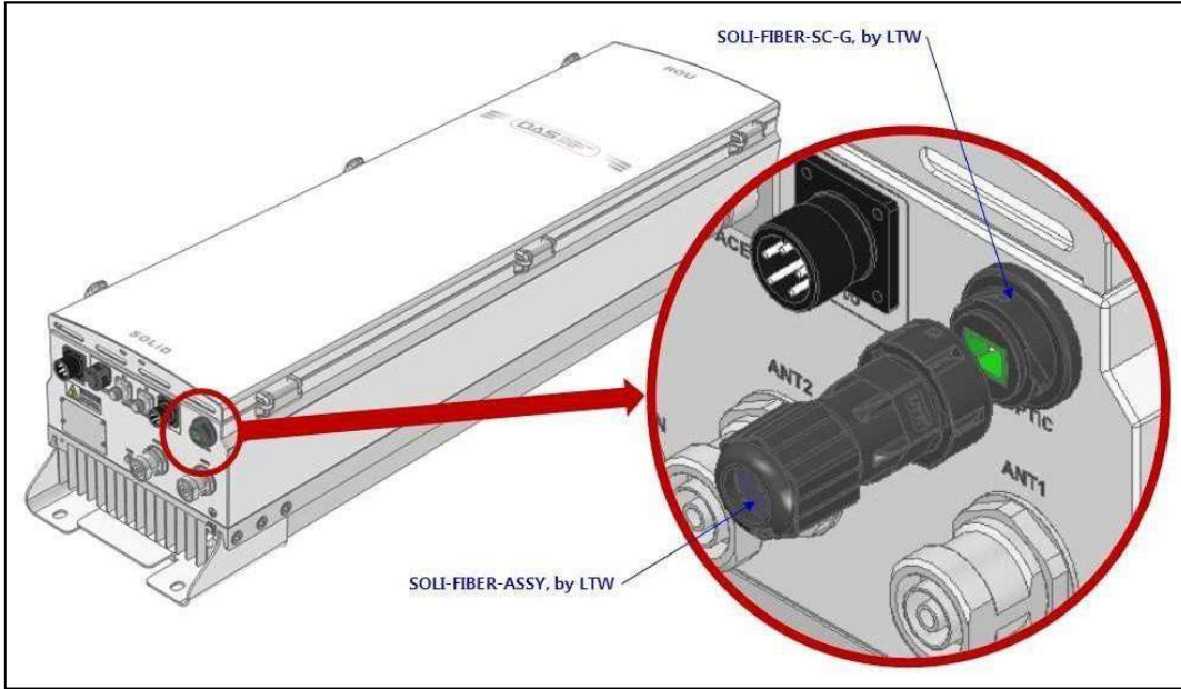
Figure 4.9 – Location of Optical Connector
