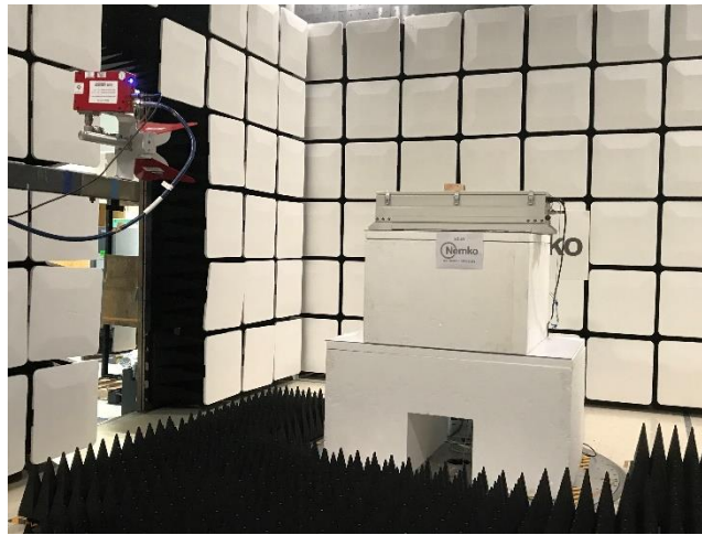
Radiated above 1GHz
