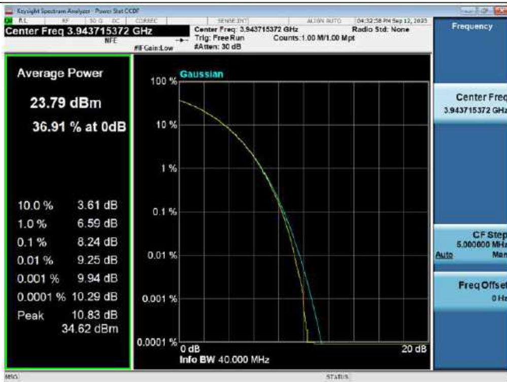
PAPR / 3.7 GHz Service (ANT 1) / Downlink / 5G NR 40 MHz
