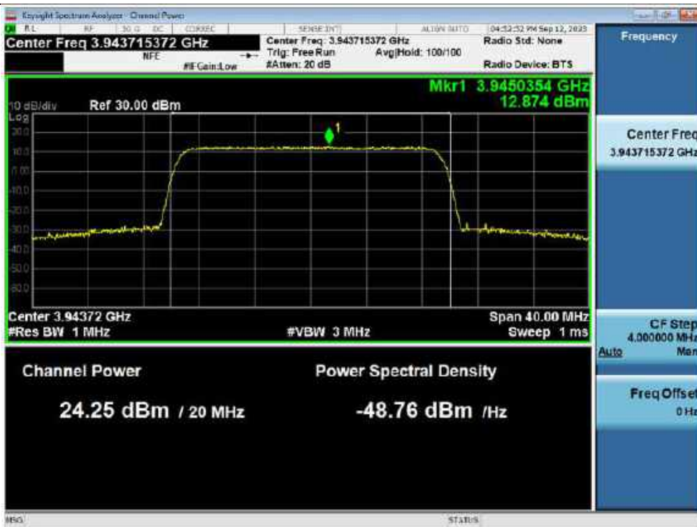
PSD / 3.7 GHz Service (ANT 1) / Downlink / 5G NR 20 MHz
