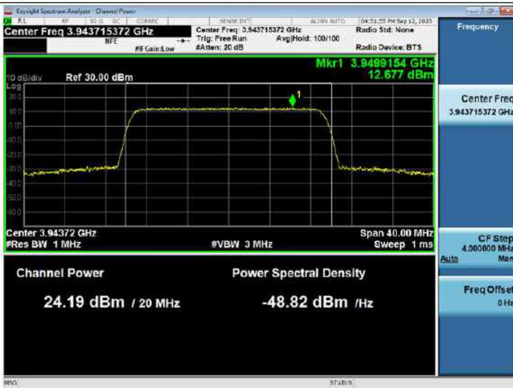
3 dB above the AGC threshold PSD / 3.7 GHz Service (ANT 1) / Downlink / 5G NR 20 MHz
