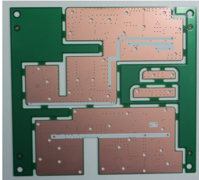
PAM PCB Bare – BOTTOM
