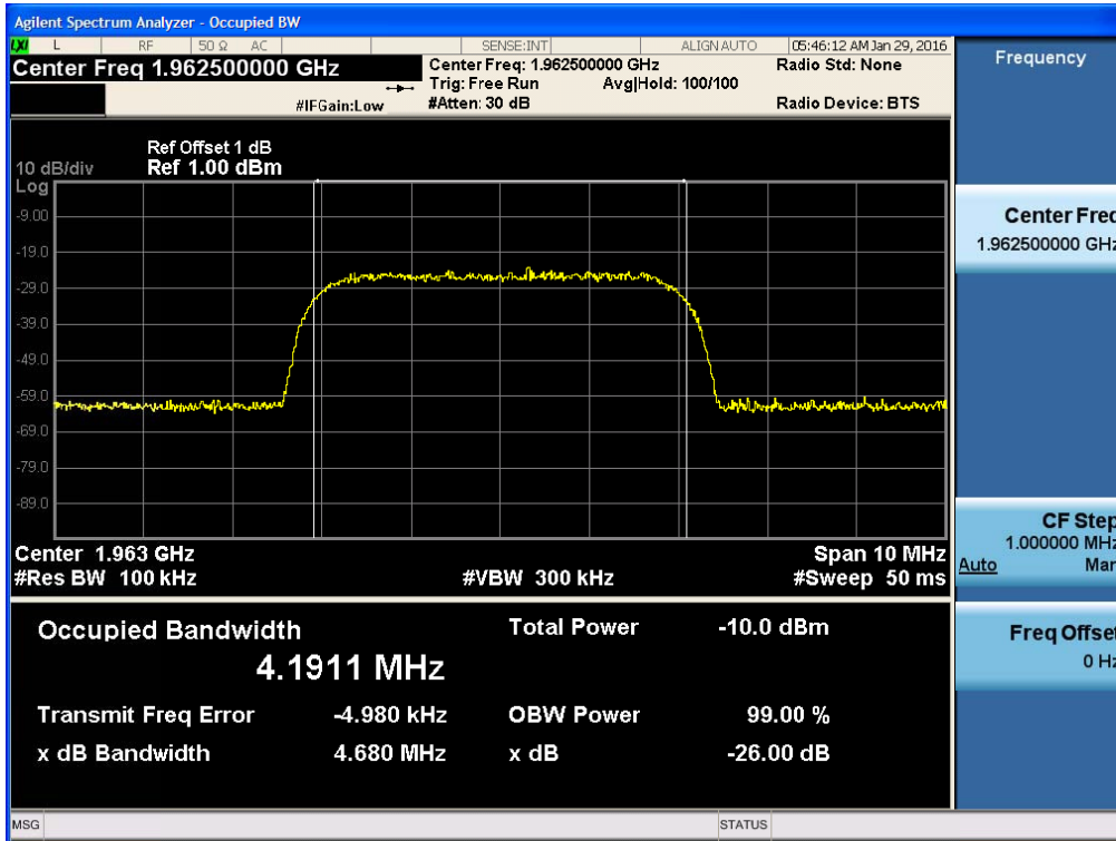
[AGC threshold Input Downlink Middle]
