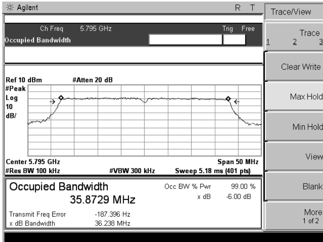
802.11a channel, 6dB bandwidth / port.1
