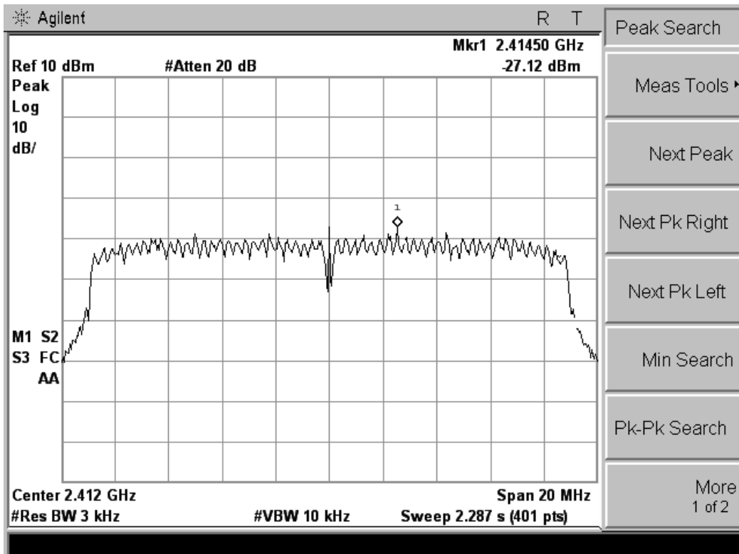
802.11n HT20 power density / port.2
