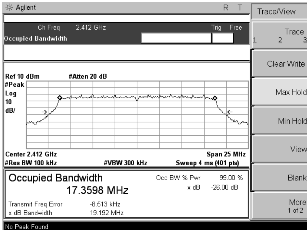
802.11n HT20 channel, 99% Occupied Bandwidth / port.1+ port.2
