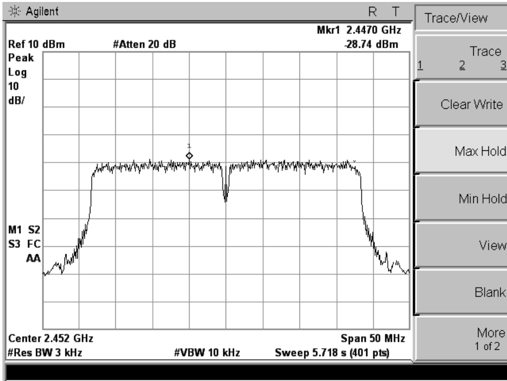
802.11n HT40 power density / port.2
