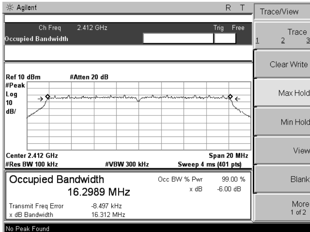
802.11g channel, 6dB bandwidth / port.1
