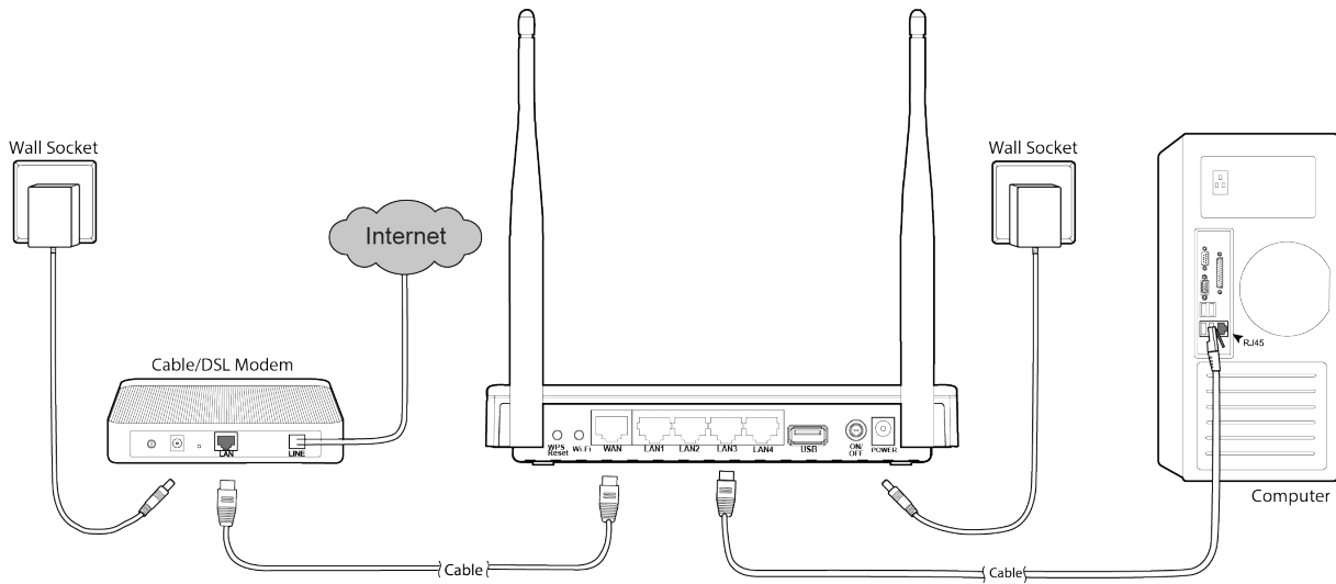
Figure 2-1 Hardware Installation
