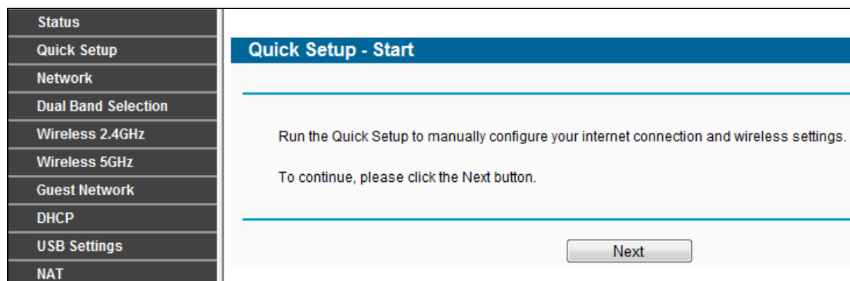
Figure 3-5 Quick Setup
