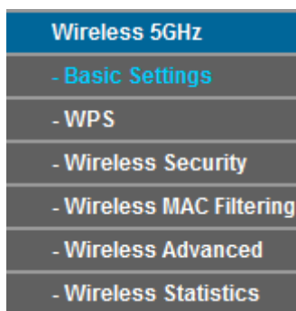
Figure 4-27 Wireless menu
