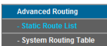
Figure 4-85 Advanced Routing
