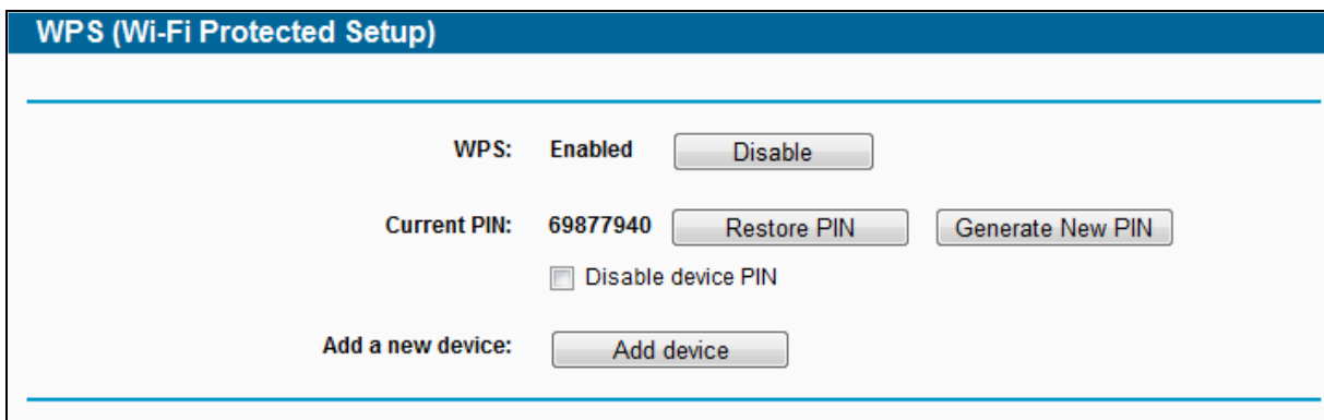
Figure 4-30 WPS
