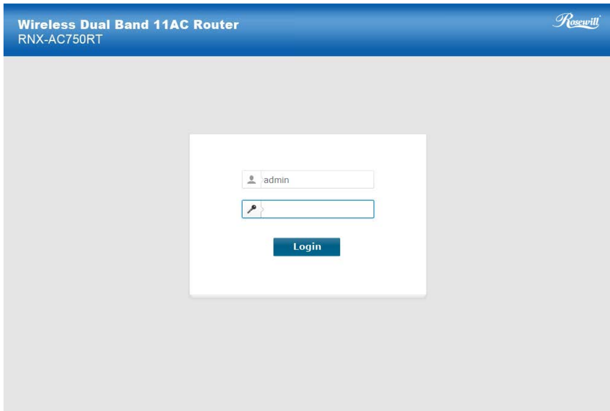
Figure 4-117 Logout
