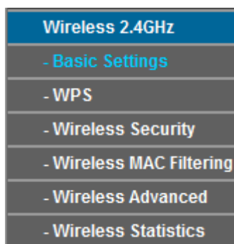
Figure 4-12 Wireless menu
