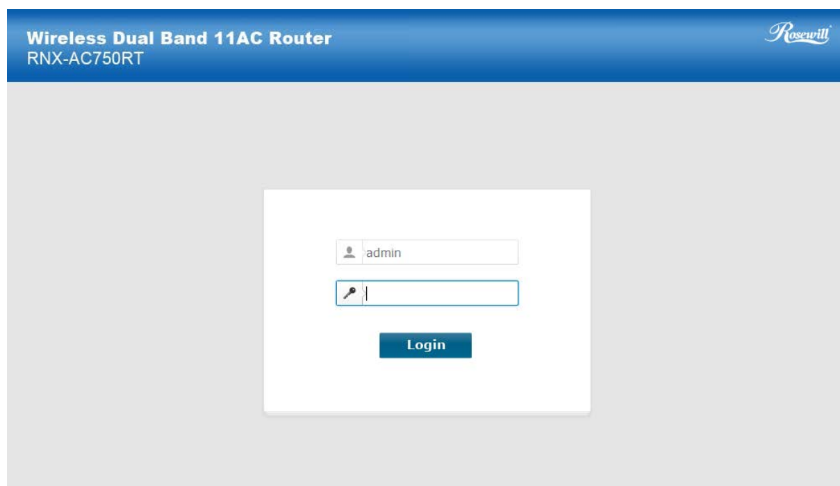
Figure 3-4 Login Windows
