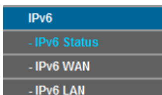
Figure 4-98 IPv6 Support
