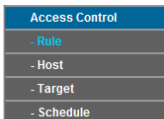
Figure 4-73 Access Control
