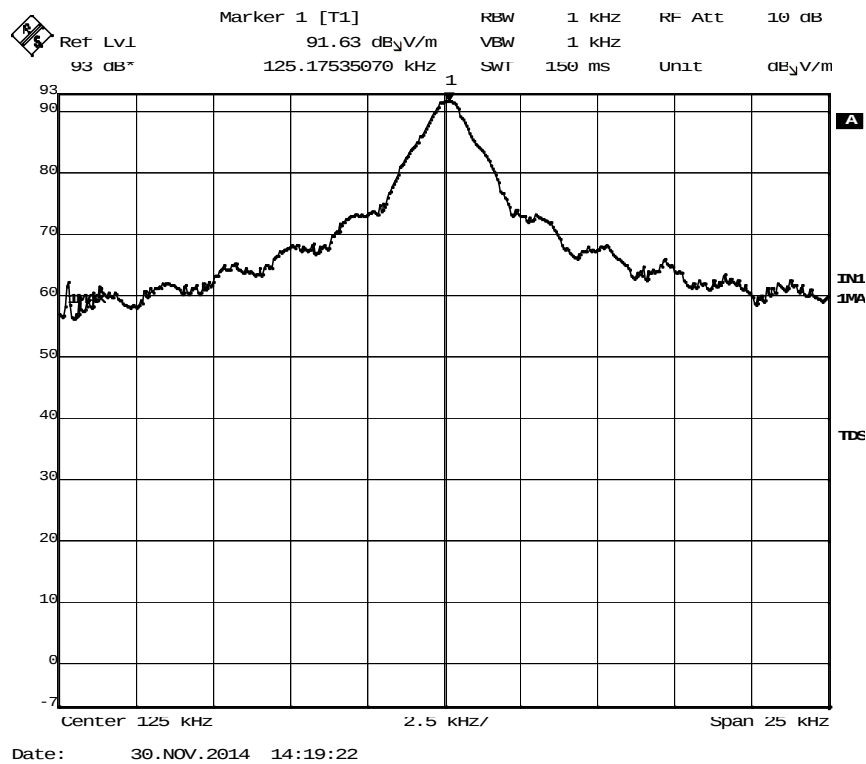
Figure 15. Field Strength of Fundamental Detector: Peak, Internal Antenna
