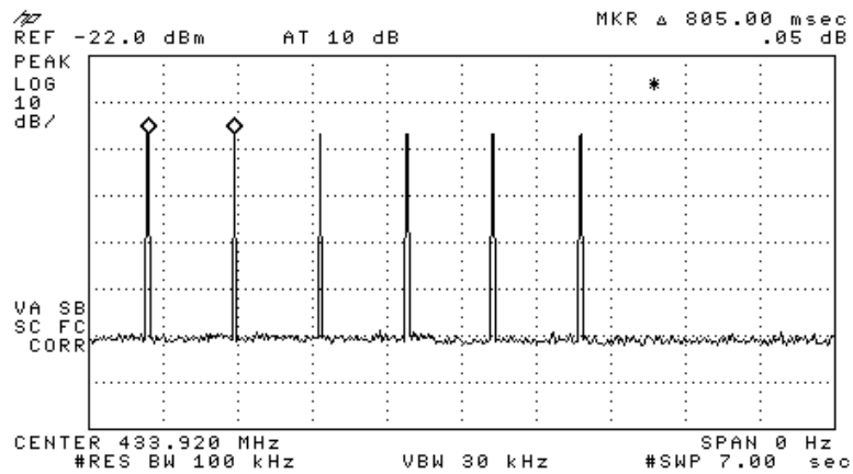
Figure 4. Burst duration = 6.5msec
