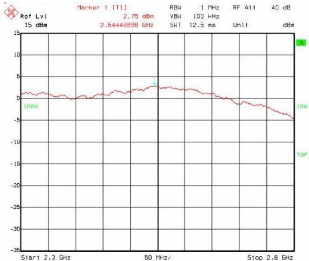
Figure 8:OUTPUT POWER,ESP-WROOM-02
