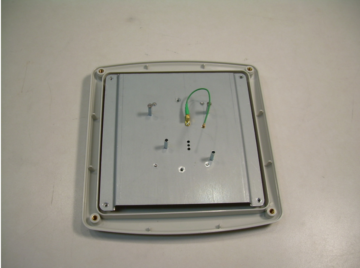
Photograph 7 – Rear Cover Removed Showing Antenna Mounting and Coax
