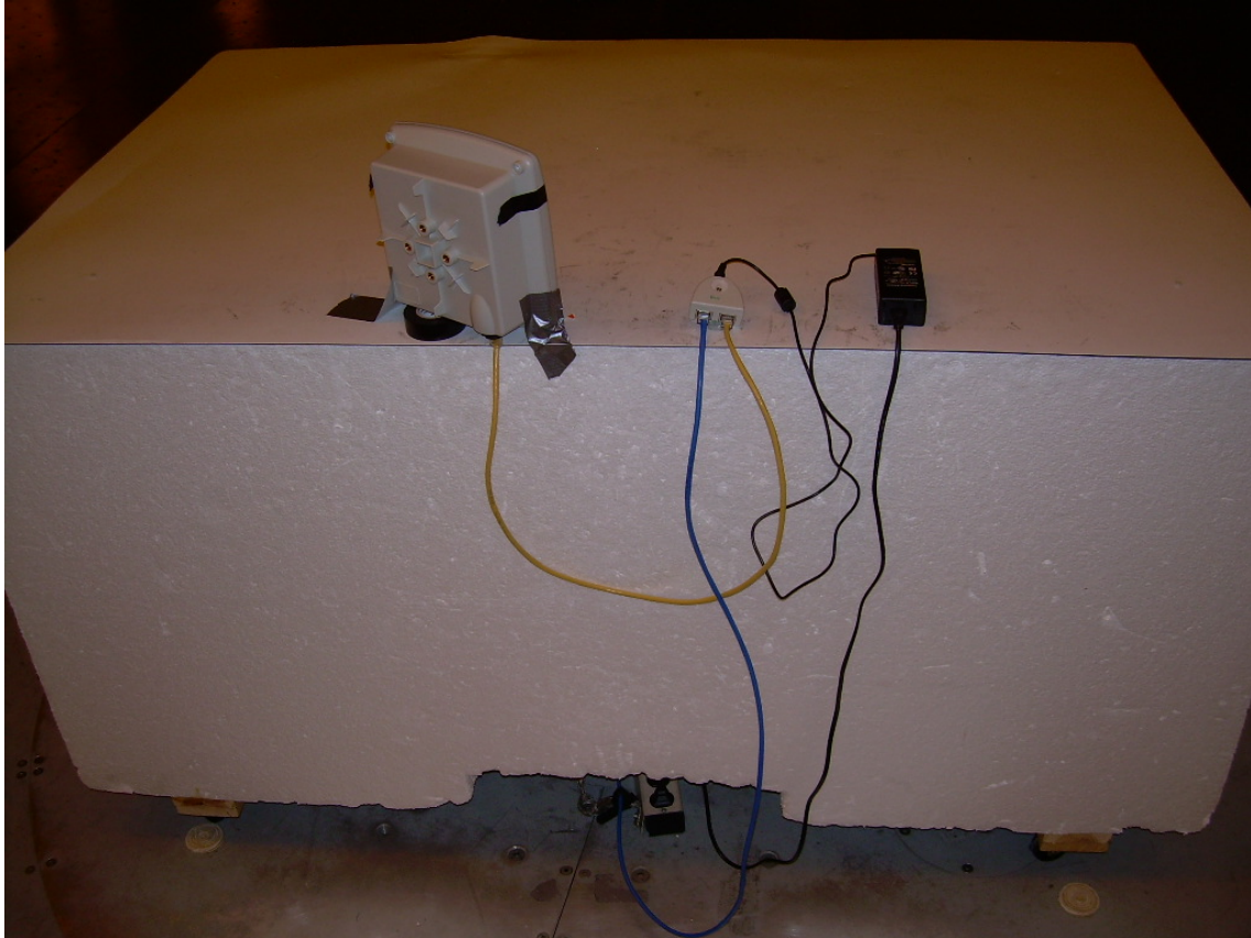
Photograph 2 – Back View Worst-Case Radiated Emissions Configuration
