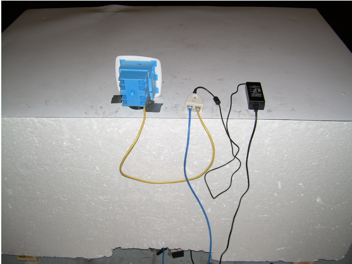
Photograph 2 – Back View Worst-Case Radiated Emissions Configuration – XAP-1010
