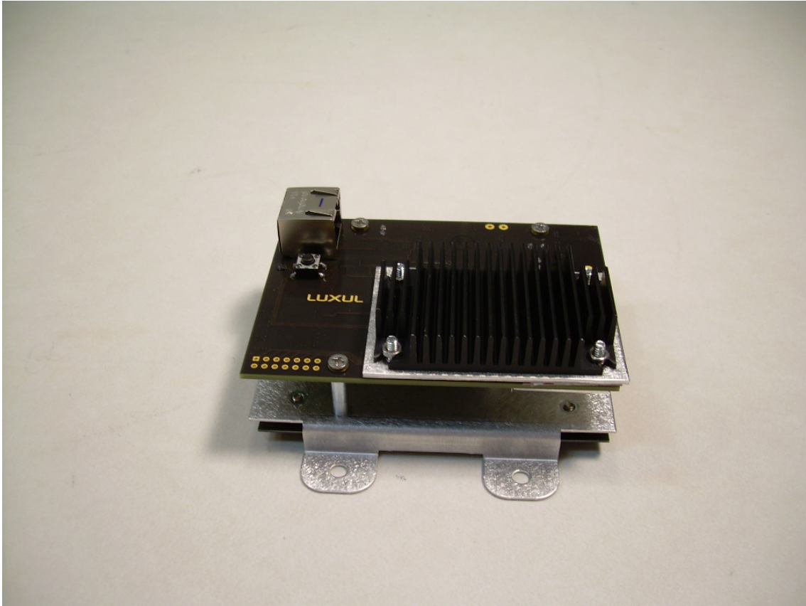
Photograph 13 – View of the Antenna/PCB Stack
