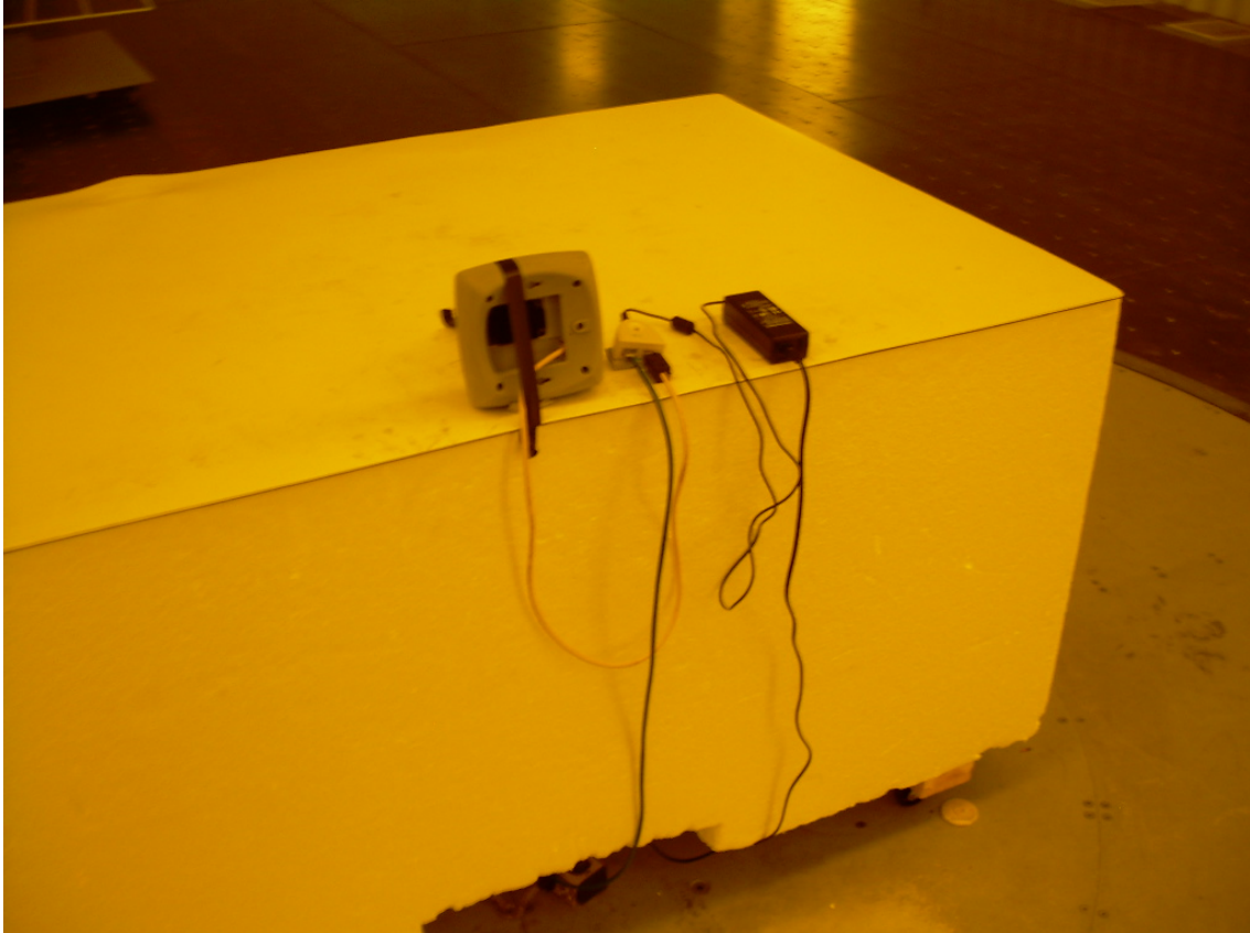
Photograph 6 – Back View Worst-Case Radiated Emissions Configuration – XAP-1020
