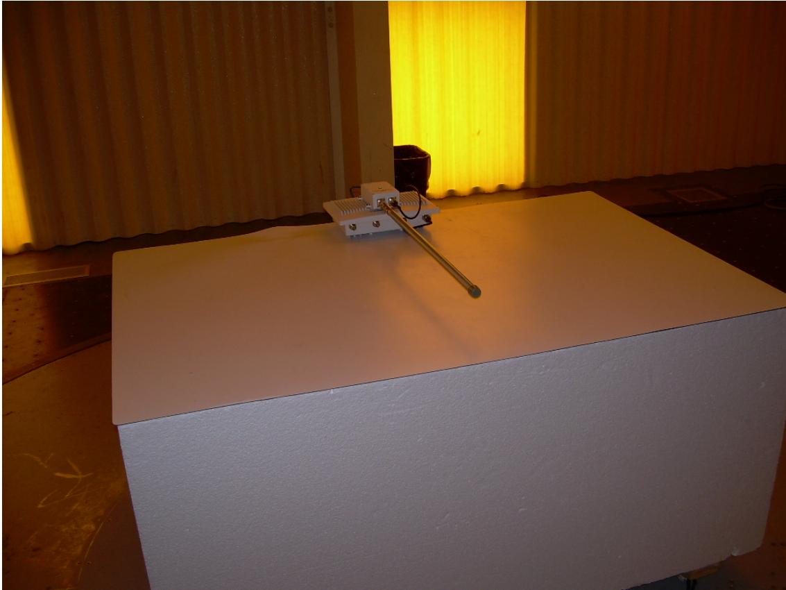
Front View Radiated Spurious Emissions Test Set-up Using the Motorola OD24M-9 Antenna
