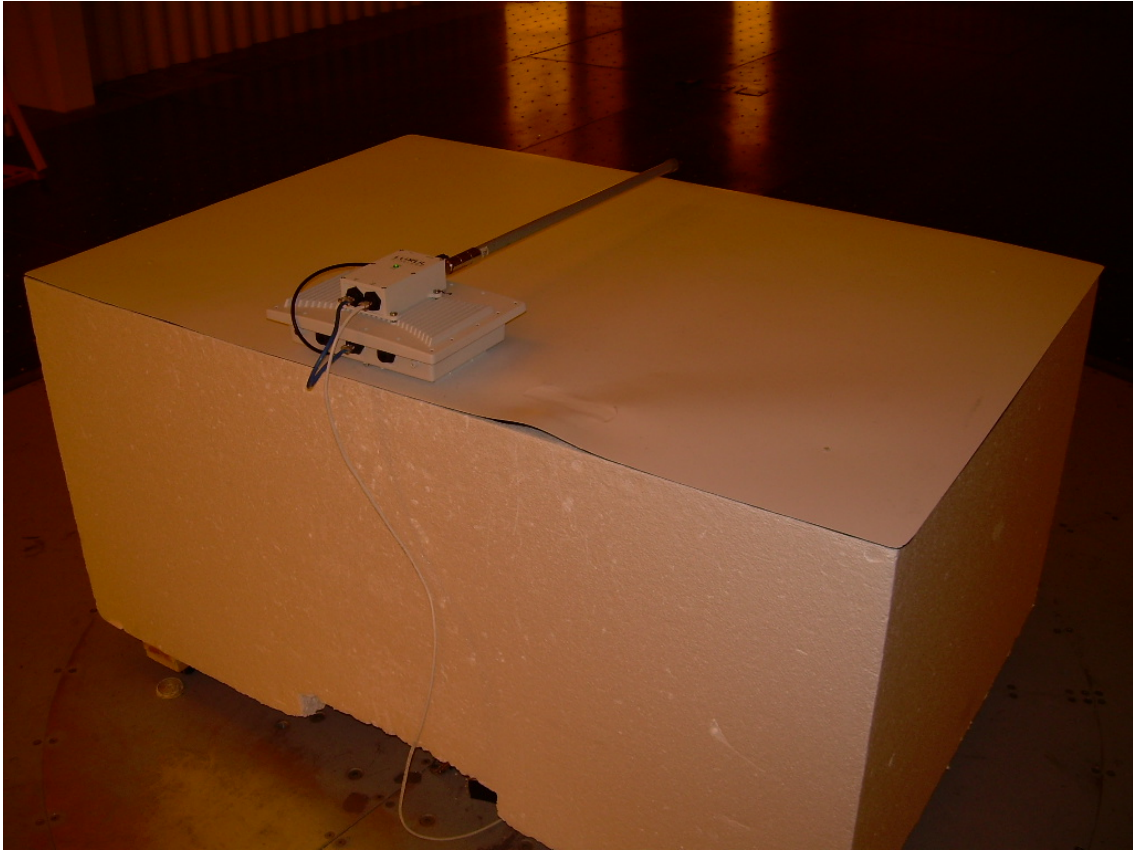
Back View Radiated Spurious Emissions Test Set-up Using the Motorola OD24M-9 Antenna
