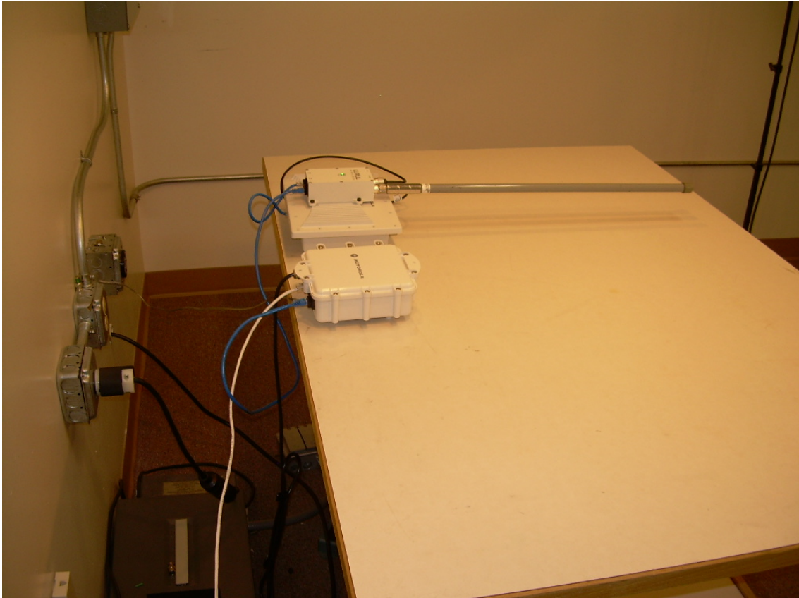
Back View Conducted Emissions Worst Case Configuration
