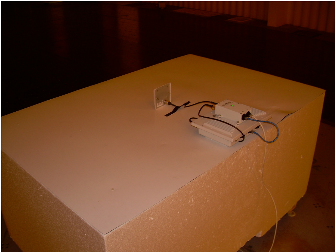
Back View of Radiated Spurious Emission Testing Set-up with Luxul XW-24-FP7 Antenna
