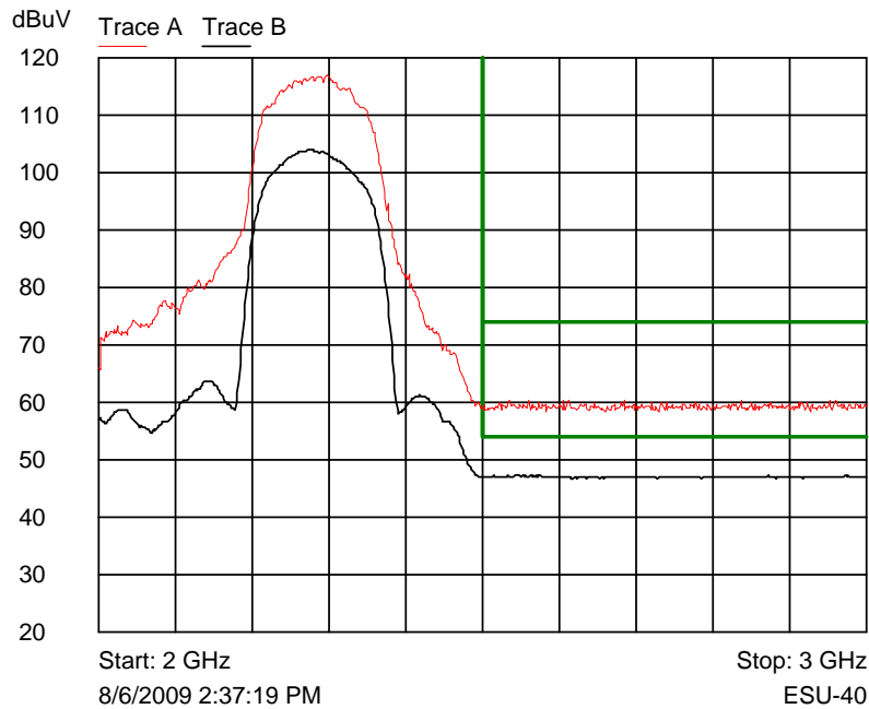
5 dbi antenna Mode B 11 Mb Trace A Peak upper Band edge Trace B Average upper band edge
