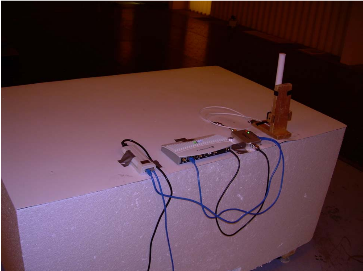
Photograph 2 - Back View Radiated Disturbance Worst Case Configuration(5 dBi Antenna)
