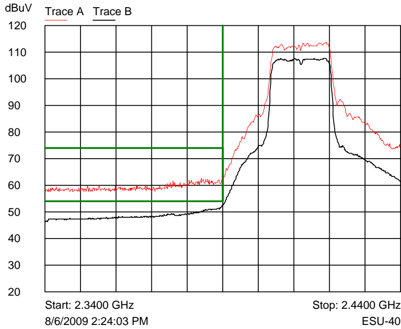
5 dbi antenna Mode G 11 Mb Trace A Peak Lower Band edge Trace B Average lower band edge
