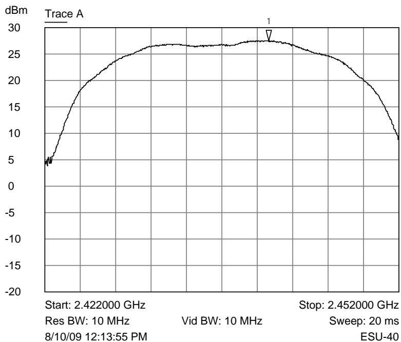
Mode G 54 Mb Trace A Middle channel Peak Power
