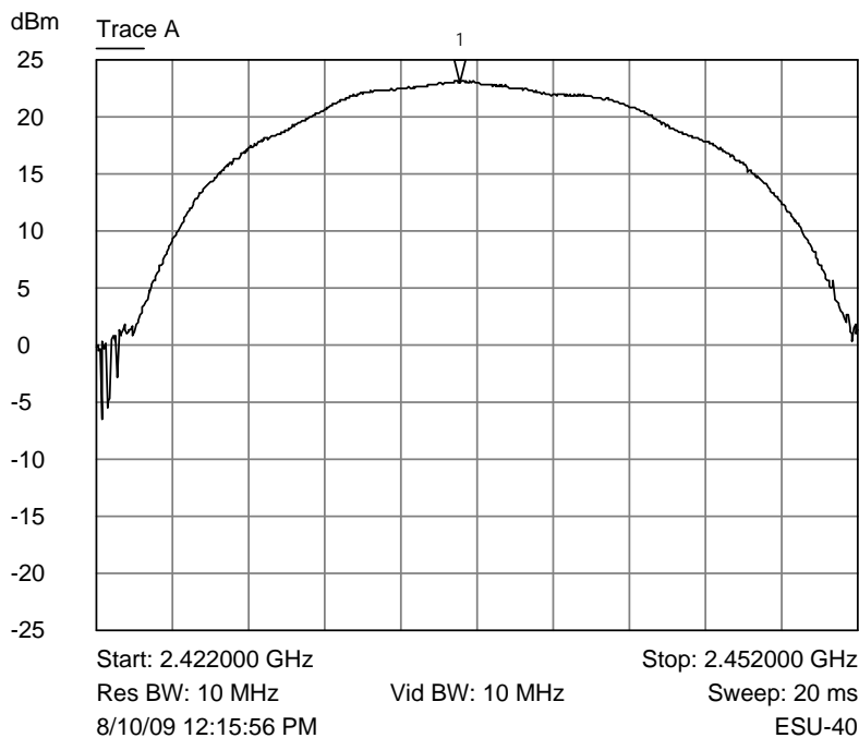
Mode B 11 Mb Trace A Middle channel Peak Power
