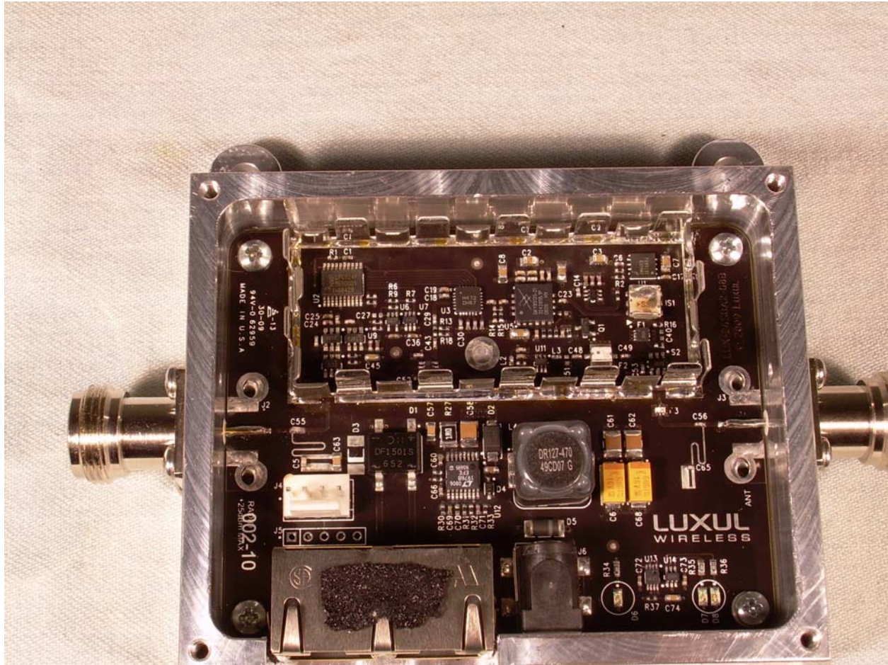
Photograph 7 - Internal View of the EUT with Shield Removed
