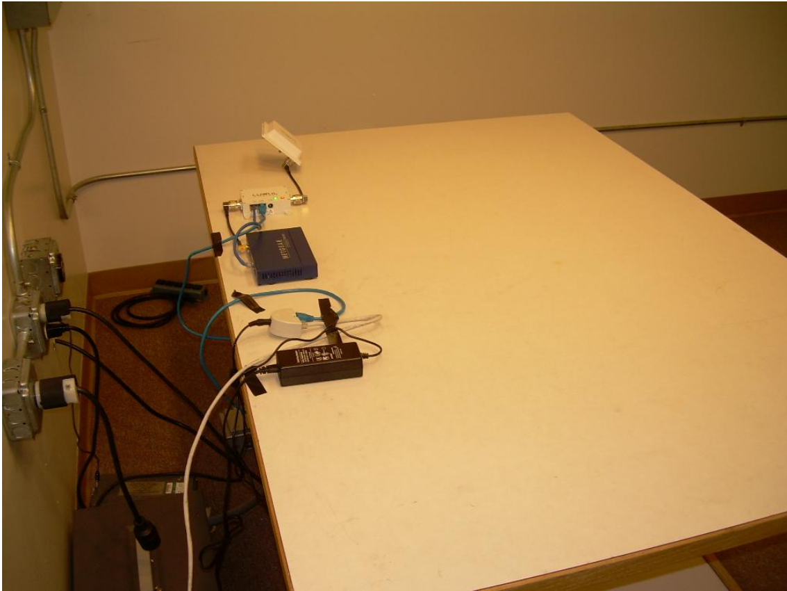
Back View of Worst-Case Conducted Emission Configuration
