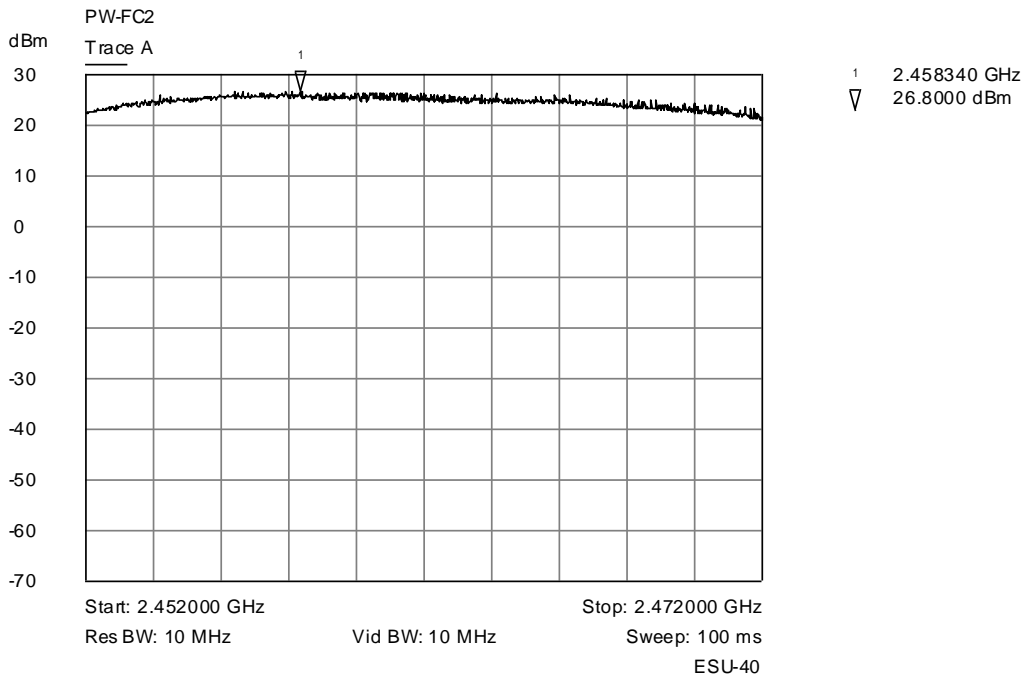
Trace A Upper channel output power plot - "G" mode - Corrected trace
