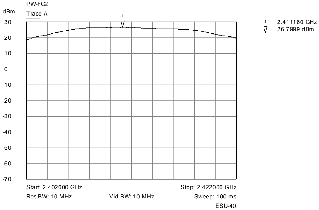
Trace A Lower channel output power plot - "B" mode - Corrected trace
