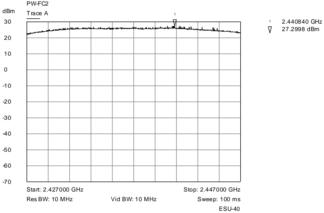
Trace A Middle channel output power plot - "G" mode - Corrected trace
