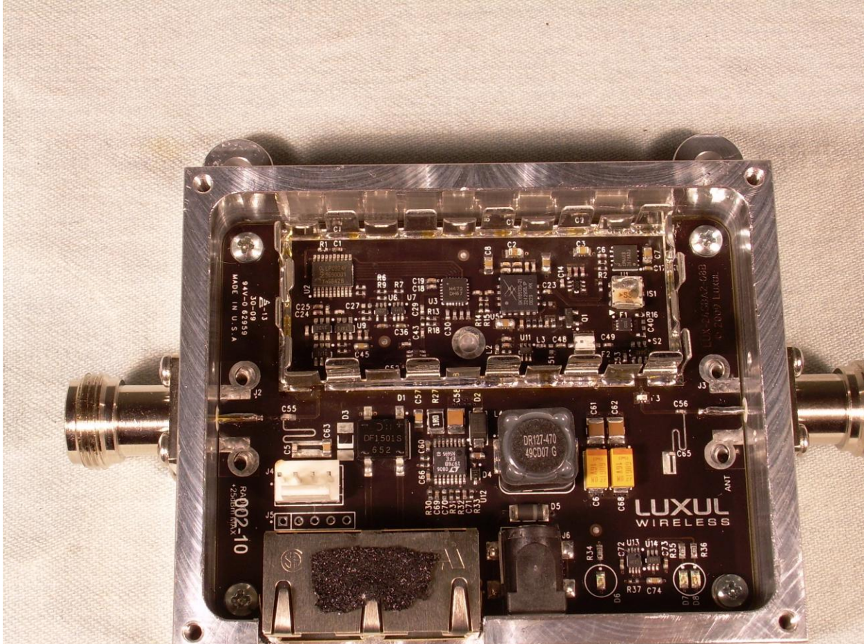
Photograph 12 – Internal View of the EUT with RF Shield Removed
