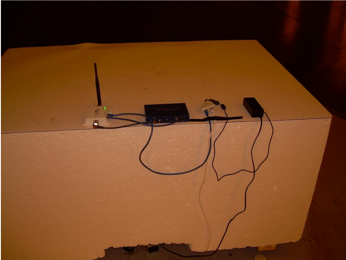
Photograph 2 – Back View Radiated Emissions Configuration Using POE Power and 5 dBi Omni Antenna
