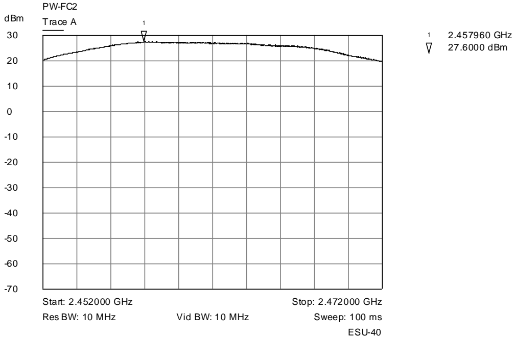
Trace A Upper channel output power plot - "B" mode - Corrected trace
