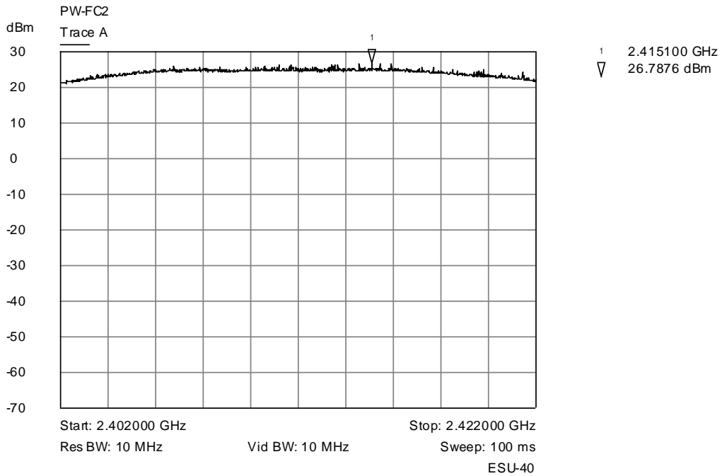
Trace A Lower channel output power plot - "G" mode - Corrected trace
