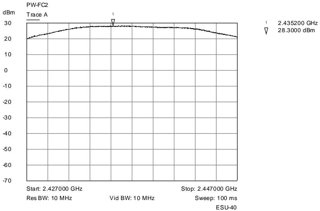
Trace A Middle channel output power plot - "B" mode - Corrected trace
