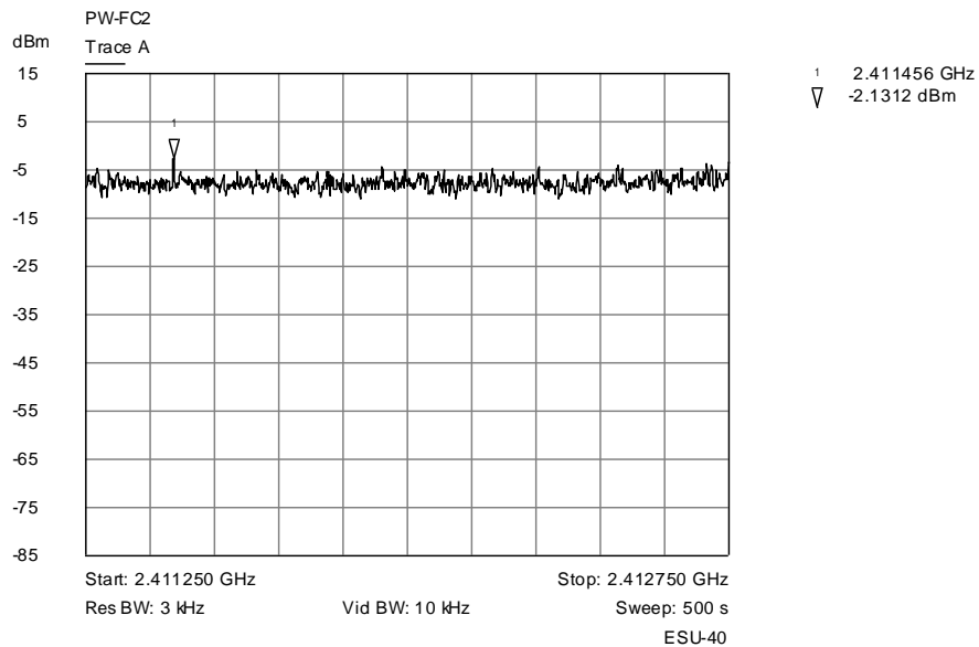
Lowest channel – 802.11b
