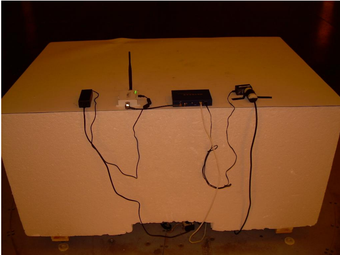
Photograph 6 – Back View Radiated Emissions Configuration Using External Power to the Access Point and 5 dBi Omni Antenna
