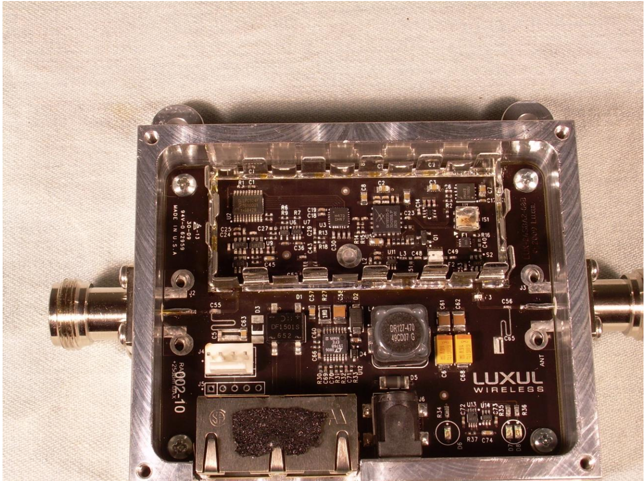
Internal View of the EUT with RF Shield Removed
