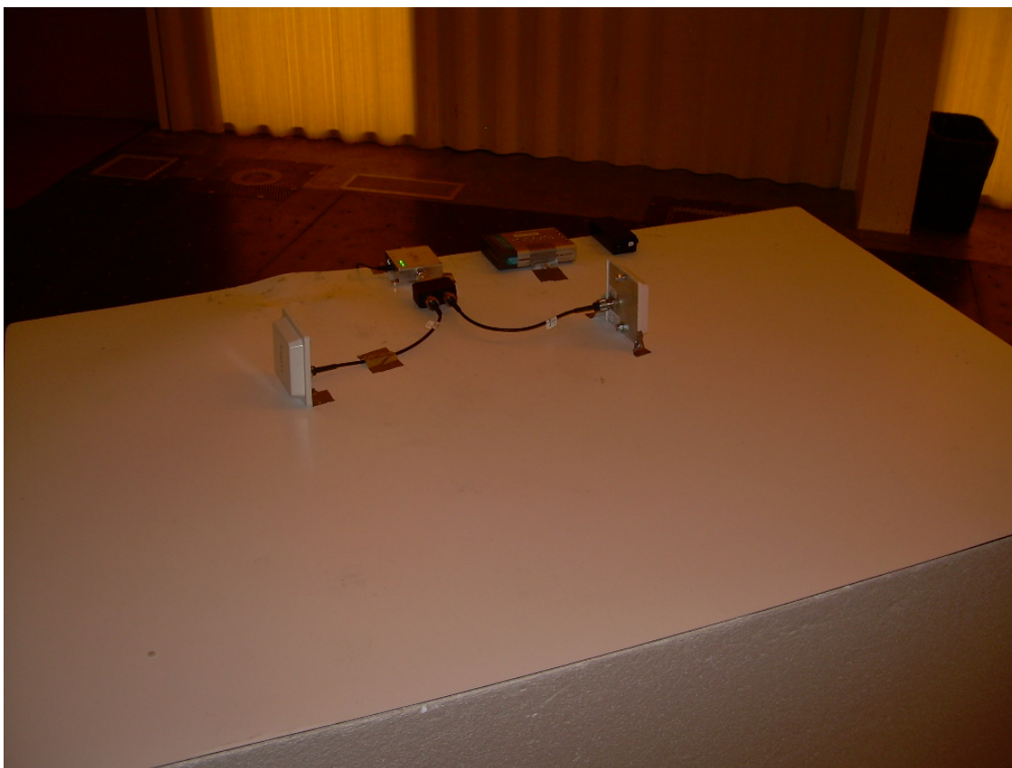
Front View of Radiated Spurious Emission Testing with Dual Antenna Configuration
