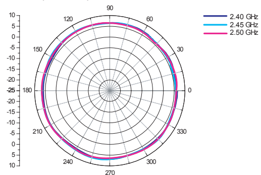
H-plane co-polarization Pattern
