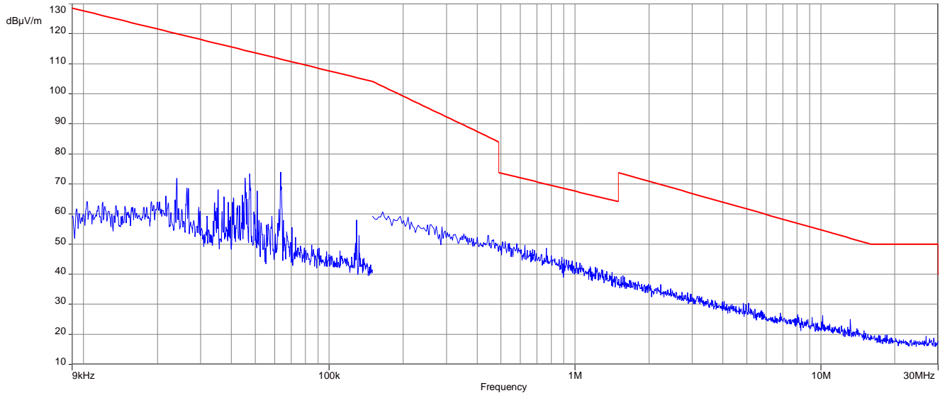
Plot 1: 9 kHz to 30 MHz, 2404 MHz, transmit mode, MSK
