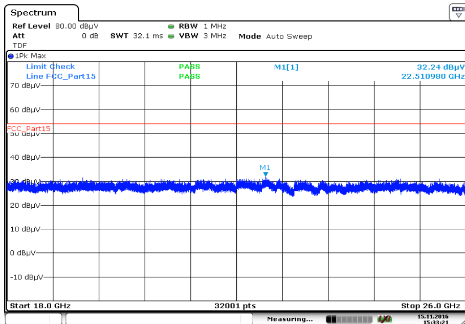
Plot 8: 18 GHz to 26 GHz, TX mode, 2447.0 MHz, vertical & horizontal polarization
