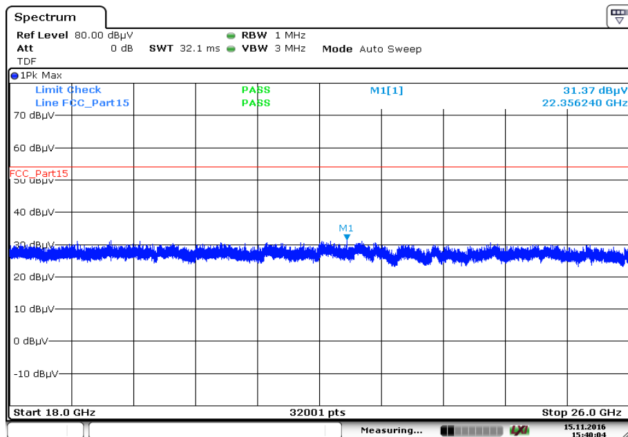
Plot 12: 18 GHz to 26 GHz, TX mode, 2479.3 MHz, vertical & horizontal polarization
