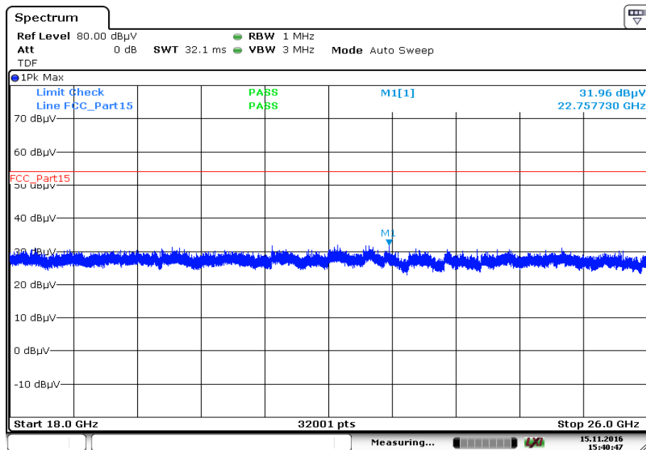
Plot 4: 18 GHz to 26 GHz, TX mode, 2404.0 MHz, vertical & horizontal polarization
