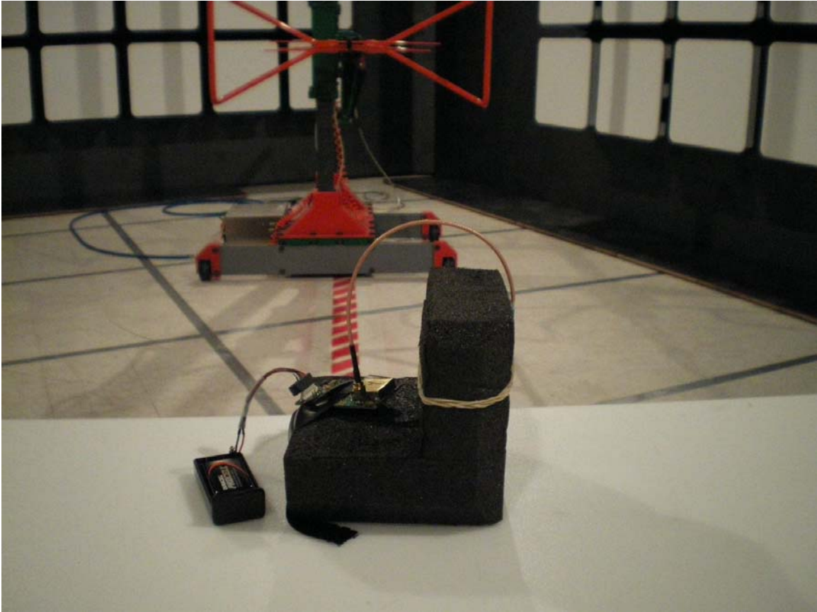
Radiated Emissions with Patch antenna
