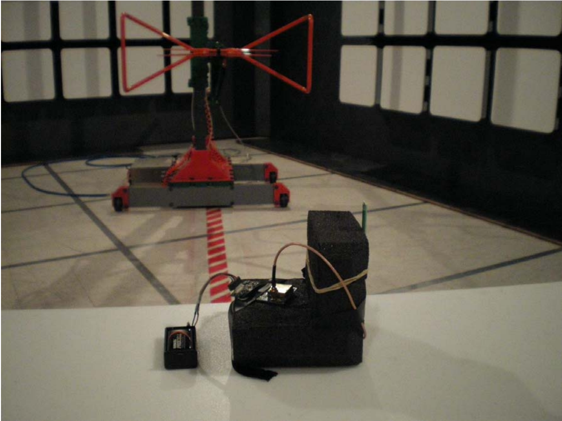
Radiated Emissions with J-Pole antenna
