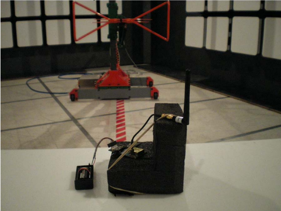
Radiated Emissions with Whip antenna
