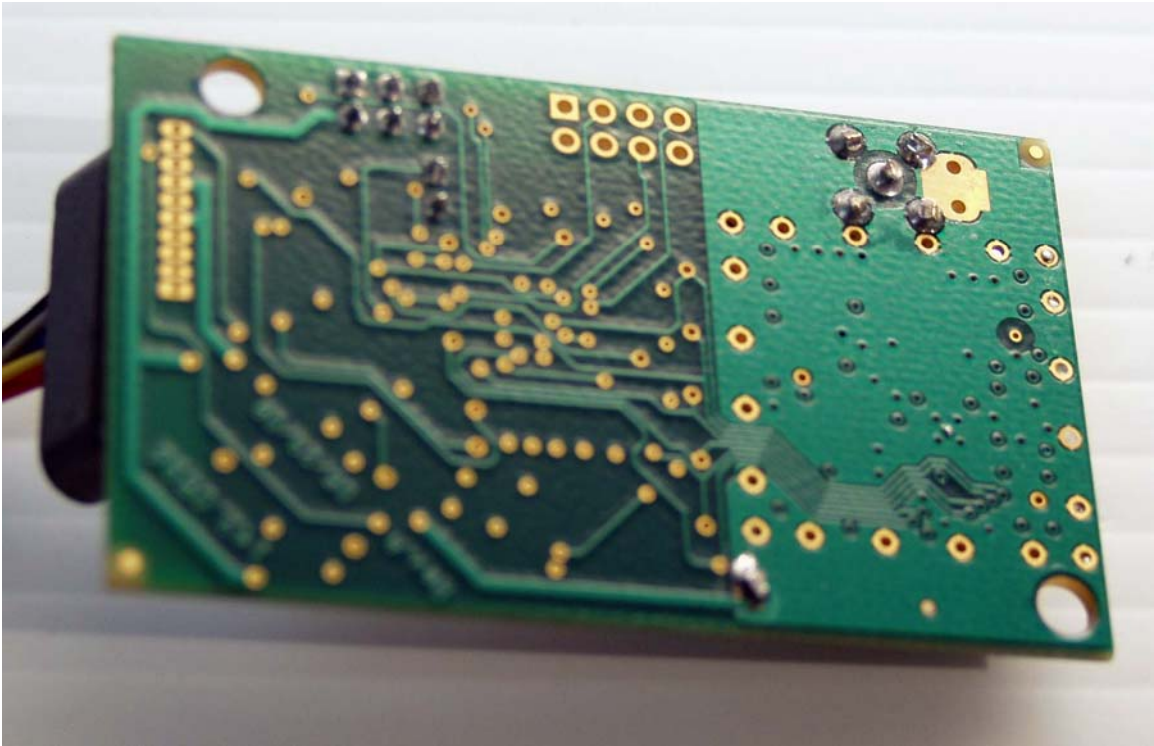
Main PCB bottom view
