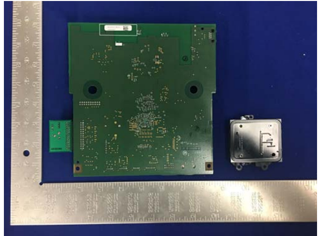
EUT View 2
