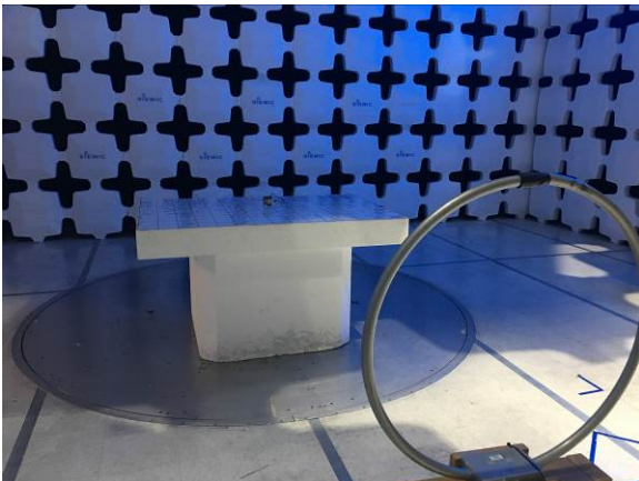
Radiated Emissions (<30MHz) – 0 Degree Angel View
