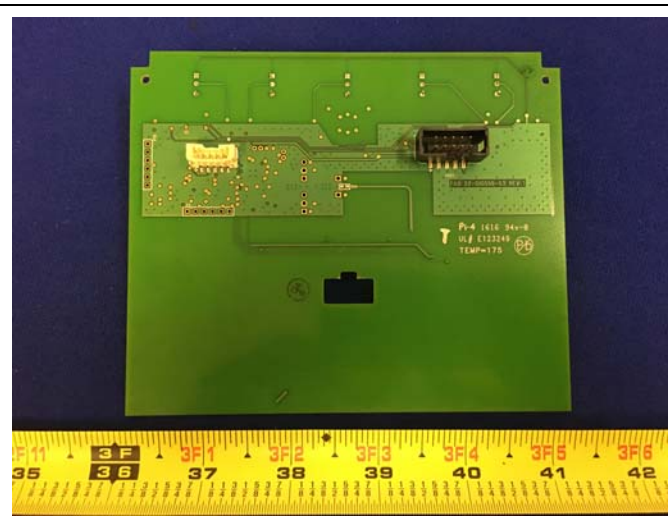
EUT-RFID Board with antenna Rear View
