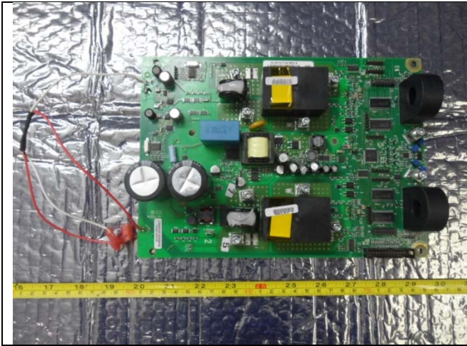
PCBA – Power Supply Top View
