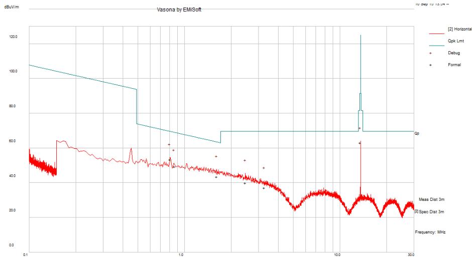
f= 100kHz – 30MHz plot, and loop antenna at 0 degree at 3m distance
