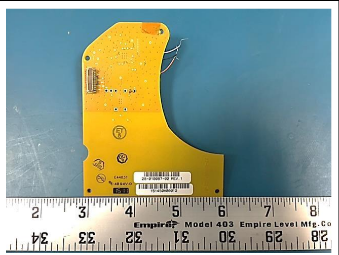
PCBA1 RFID - View 2
